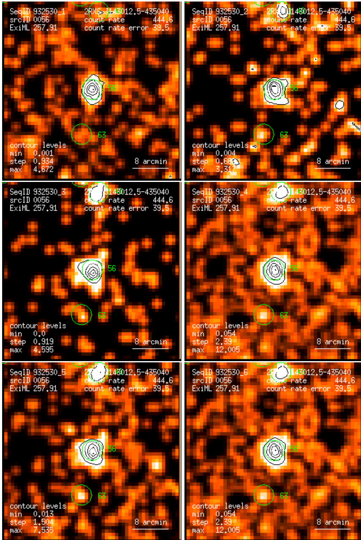
Figure 56: RASS 932530: detection 0056: band rate images, Gaussian filter: (1) PSPC channels 11 – 41, (2) 52 – 90, (3) 91 – 201, (4) 11 – 235, (5) 52 – 201, (6) 11 – 201. Broad band rates in counts/ks. Band rate contour levels in counts/ks/arcmin 2 .
