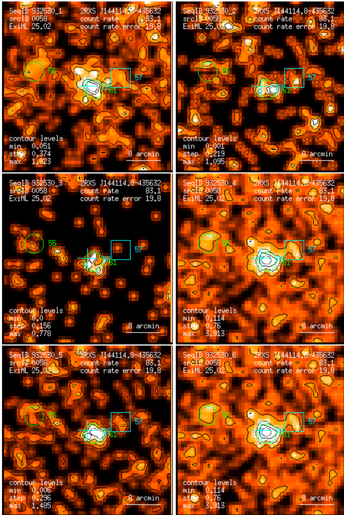
Figure 58: RASS 932530: detection 0058: band rate images, Gaussian filter: (1) PSPC channels 11 – 41, (2) 52 – 90, (3) 91 – 201, (4) 11 – 235, (5) 52 – 201, (6) 11 – 201. Broad band rates in counts/ks. Band rate contour levels in counts/ks/arcmin 2 .
