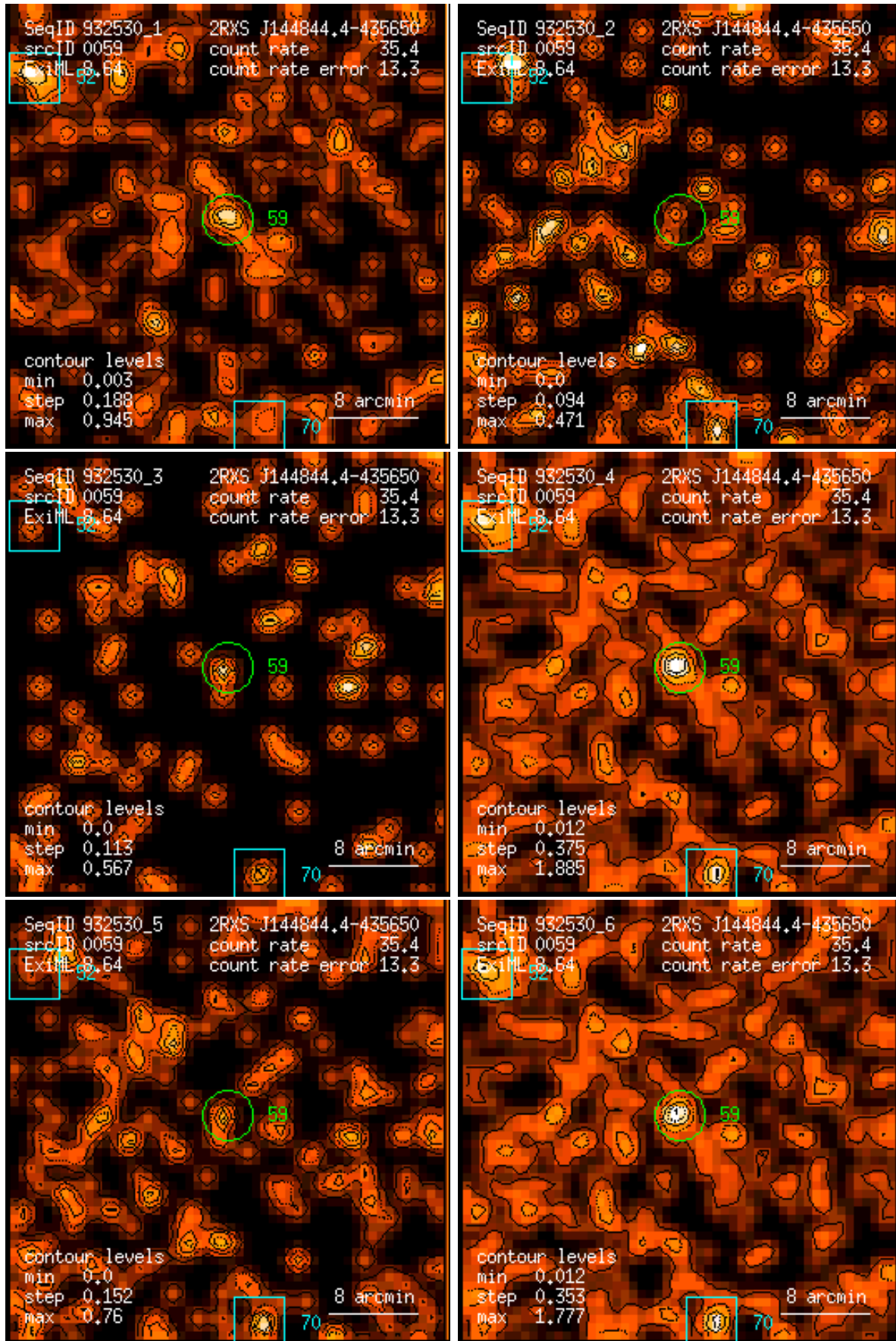
Figure 59: RASS 932530: detection 0059: band rate images, Gaussian filter: (1) PSPC channels 11 – 41, (2) 52 – 90, (3) 91 – 201, (4) 11 – 235, (5) 52 – 201, (6) 11 – 201. Broad band rates in counts/ks. Band rate contour levels in counts/ks/arcmin 2 .
