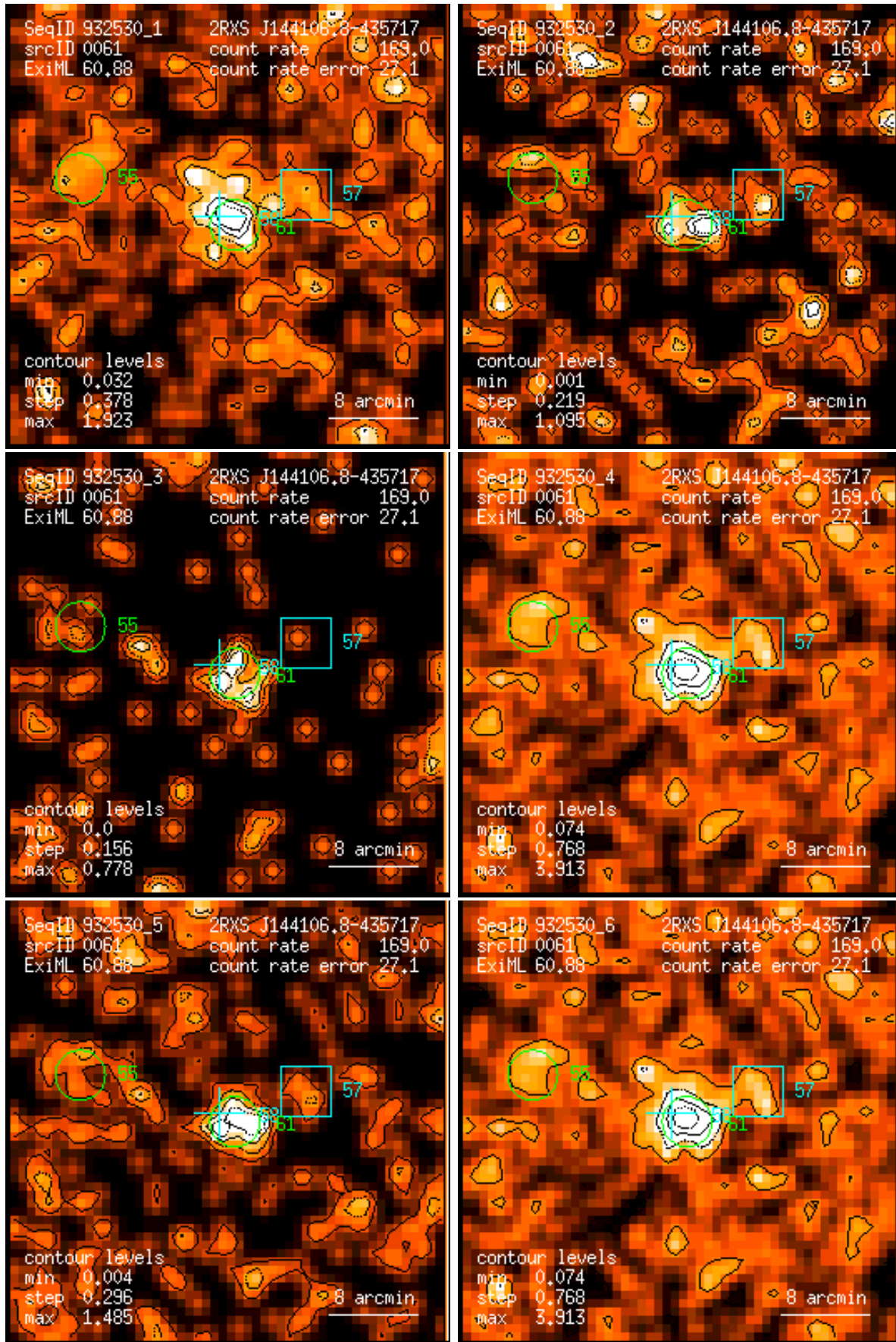
Figure 61: RASS 932530: detection 0061: band rate images, Gaussian filter: (1) PSPC channels 11 – 41, (2) 52 – 90, (3) 91 – 201, (4) 11 – 235, (5) 52 – 201, (6) 11 – 201. Broad band rates in counts/ks. Band rate contour levels in counts/ks/arcmin 2 .
