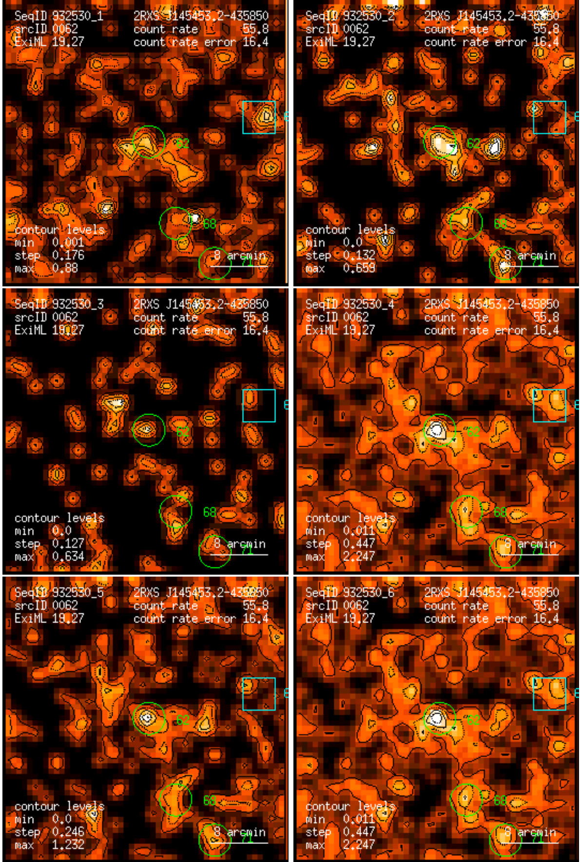
Figure 62: RASS 932530: detection 0062: band rate images, Gaussian filter: (1) PSPC channels 11 – 41, (2) 52 – 90, (3) 91 – 201, (4) 11 – 235, (5) 52 – 201, (6) 11 – 201. Broad band rates in counts/ks. Band rate contour levels in counts/ks/arcmin 2 .
