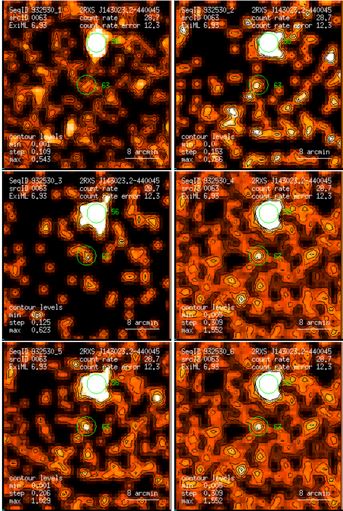
Figure 63: RASS 932530: detection 0063: band rate images, Gaussian filter: (1) PSPC channels 11 – 41, (2) 52 – 90, (3) 91 – 201, (4) 11 – 235, (5) 52 – 201, (6) 11 – 201. Broad band rates in counts/ks. Band rate contour levels in counts/ks/arcmin 2 .
