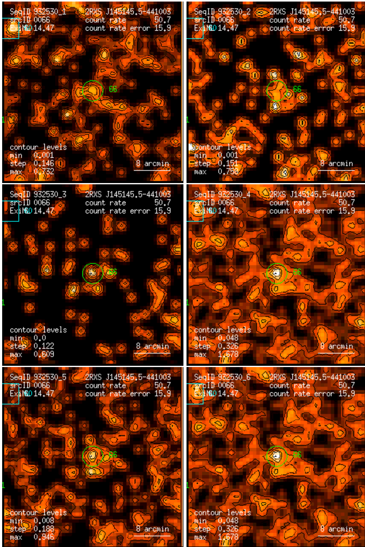
Figure 66: RASS 932530: detection 0066: band rate images, Gaussian filter: (1) PSPC channels 11 – 41, (2) 52 – 90, (3) 91 – 201, (4) 11 – 235, (5) 52 – 201, (6) 11 – 201. Broad band rates in counts/ks. Band rate contour levels in counts/ks/arcmin 2 .
