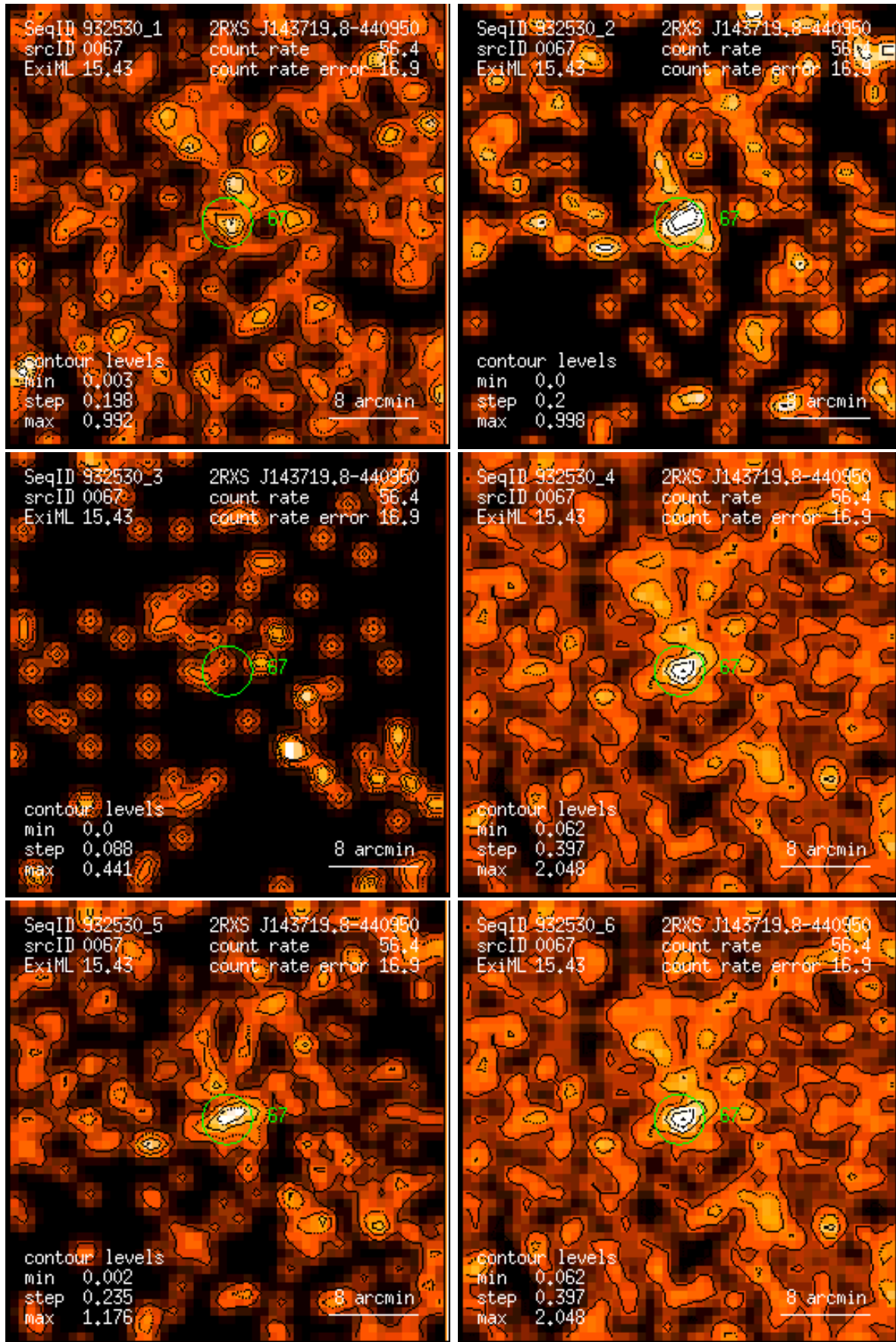
Figure 67: RASS 932530: detection 0067: band rate images, Gaussian filter: (1) PSPC channels 11 – 41, (2) 52 – 90, (3) 91 – 201, (4) 11 – 235, (5) 52 – 201, (6) 11 – 201. Broad band rates in counts/ks. Band rate contour levels in counts/ks/arcmin 2 .
