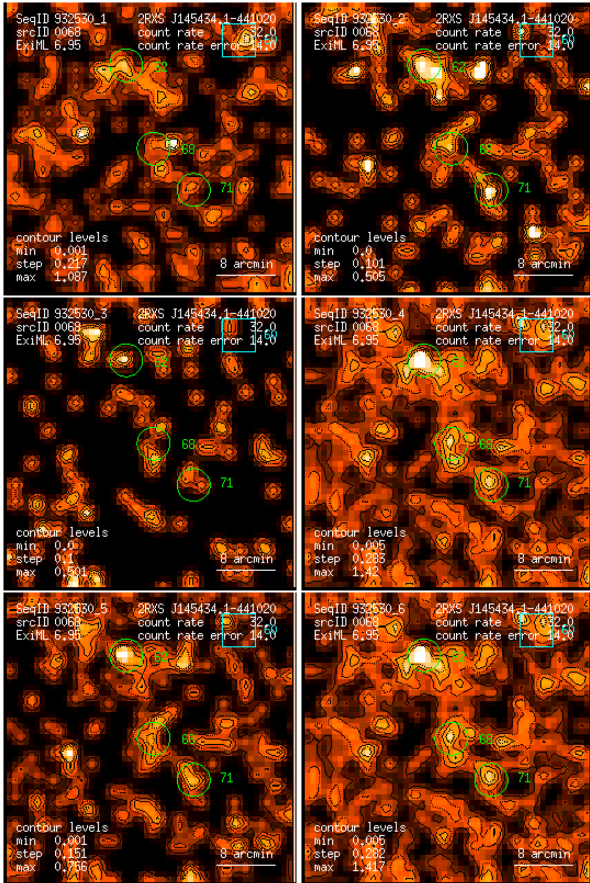
Figure 68: RASS 932530: detection 0068: band rate images, Gaussian filter: (1) PSPC channels 11 – 41, (2) 52 – 90, (3) 91 – 201, (4) 11 – 235, (5) 52 – 201, (6) 11 – 201. Broad band rates in counts/ks. Band rate contour levels in counts/ks/arcmin 2 .
