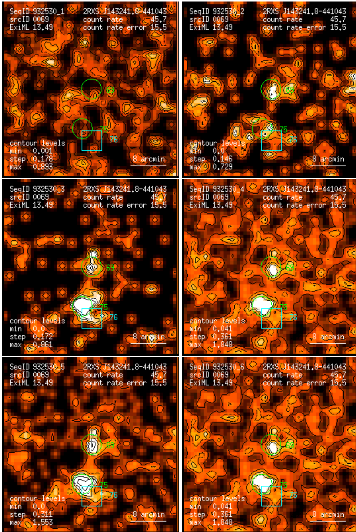
Figure 69: RASS 932530: detection 0069: band rate images, Gaussian filter: (1) PSPC channels 11 – 41, (2) 52 – 90, (3) 91 – 201, (4) 11 – 235, (5) 52 – 201, (6) 11 – 201. Broad band rates in counts/ks. Band rate contour levels in counts/ks/arcmin 2 .
