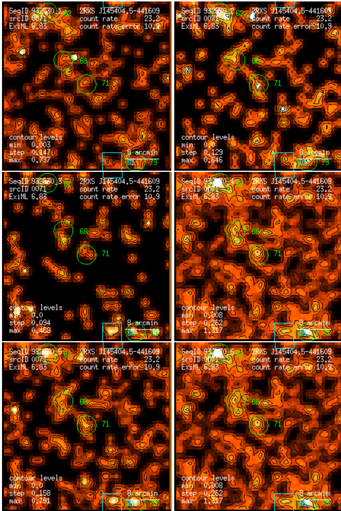
Figure 71: RASS 932530: detection 0071: band rate images, Gaussian filter: (1) PSPC channels 11 – 41, (2) 52 – 90, (3) 91 – 201, (4) 11 – 235, (5) 52 – 201, (6) 11 – 201. Broad band rates in counts/ks. Band rate contour levels in counts/ks/arcmin 2 .
