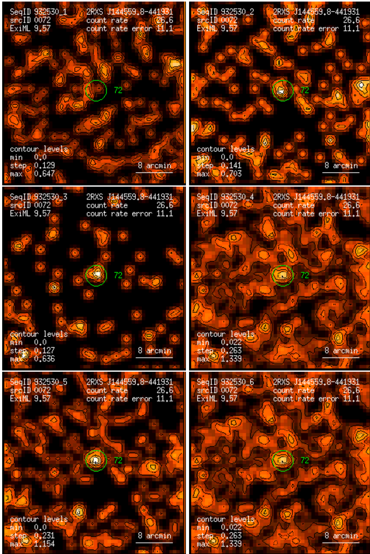
Figure 72: RASS 932530: detection 0072: band rate images, Gaussian filter: (1) PSPC channels 11 – 41, (2) 52 – 90, (3) 91 – 201, (4) 11 – 235, (5) 52 – 201, (6) 11 – 201. Broad band rates in counts/ks. Band rate contour levels in counts/ks/arcmin 2 .
