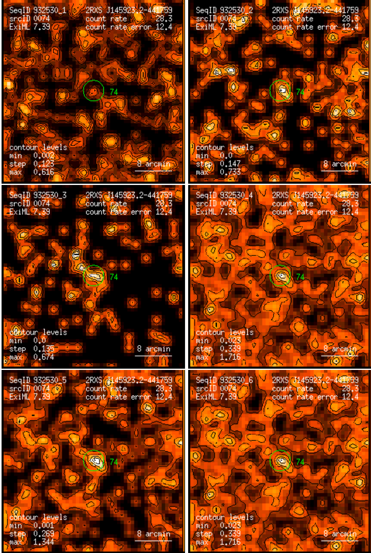
Figure 74: RASS 932530: detection 0074: band rate images, Gaussian filter: (1) PSPC channels 11 – 41, (2) 52 – 90, (3) 91 – 201, (4) 11 – 235, (5) 52 – 201, (6) 11 – 201. Broad band rates in counts/ks. Band rate contour levels in counts/ks/arcmin 2 .
