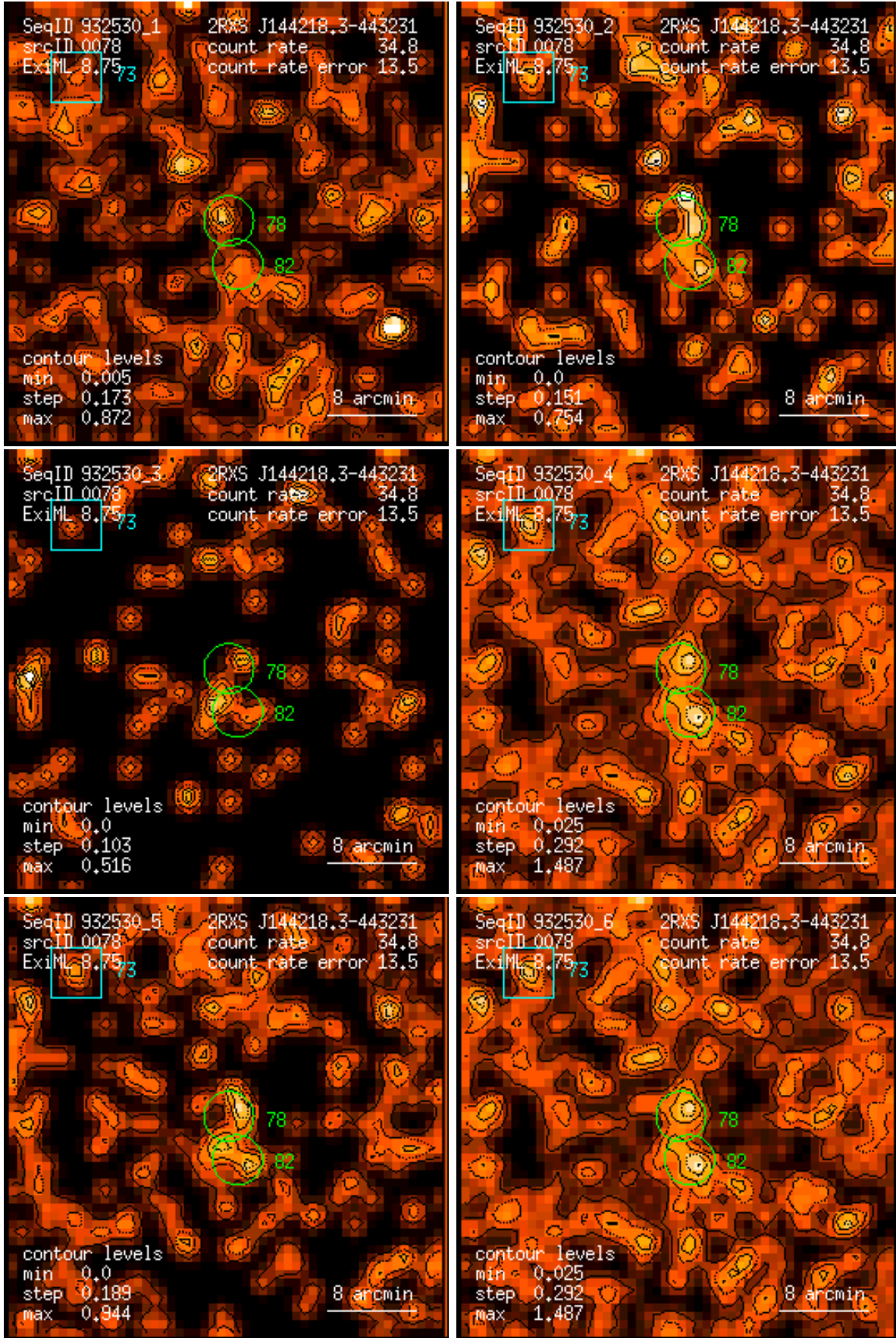
Figure 78: RASS 932530: detection 0078: band rate images, Gaussian filter: (1) PSPC channels 11 – 41, (2) 52 – 90, (3) 91 – 201, (4) 11 – 235, (5) 52 – 201, (6) 11 – 201. Broad band rates in counts/ks. Band rate contour levels in counts/ks/arcmin 2 .
