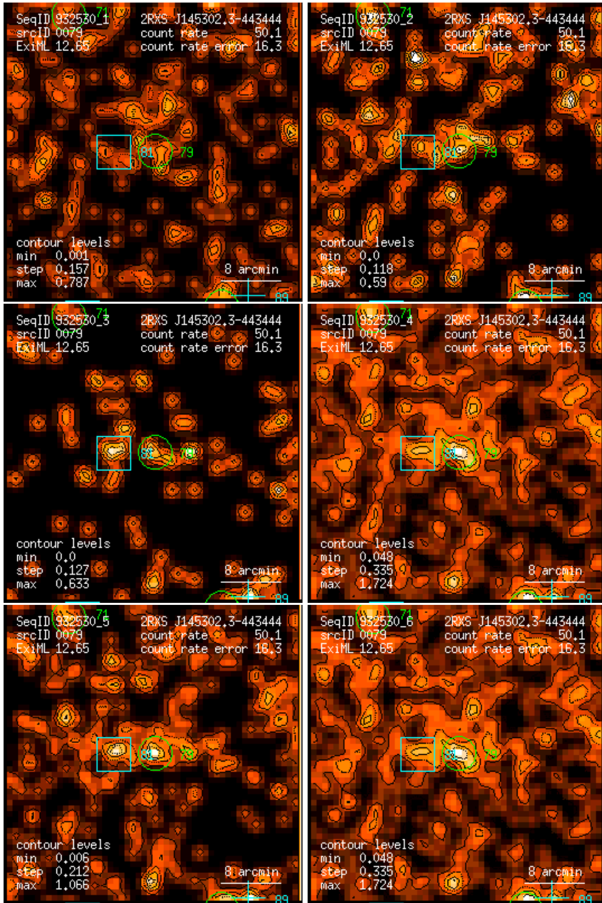
Figure 79: RASS 932530: detection 0079: band rate images, Gaussian filter: (1) PSPC channels 11 – 41, (2) 52 – 90, (3) 91 – 201, (4) 11 – 235, (5) 52 – 201, (6) 11 – 201. Broad band rates in counts/ks. Band rate contour levels in counts/ks/arcmin 2 .
