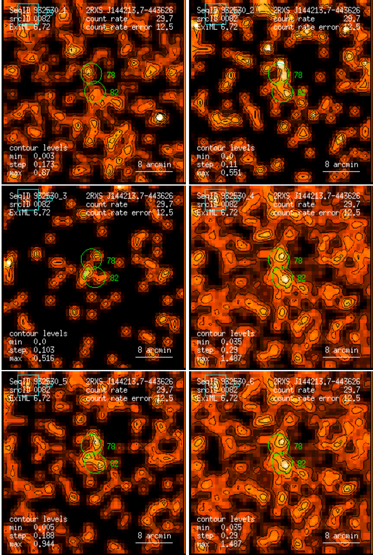
Figure 82: RASS 932530: detection 0082: band rate images, Gaussian filter: (1) PSPC channels 11 – 41, (2) 52 – 90, (3) 91 – 201, (4) 11 – 235, (5) 52 – 201, (6) 11 – 201. Broad band rates in counts/ks. Band rate contour levels in counts/ks/arcmin 2 .
