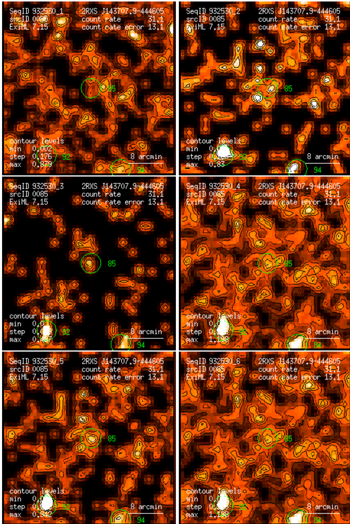
Figure 85: RASS 932530: detection 0085: band rate images, Gaussian filter: (1) PSPC channels 11 – 41, (2) 52 – 90, (3) 91 – 201, (4) 11 – 235, (5) 52 – 201, (6) 11 – 201. Broad band rates in counts/ks. Band rate contour levels in counts/ks/arcmin 2 .
