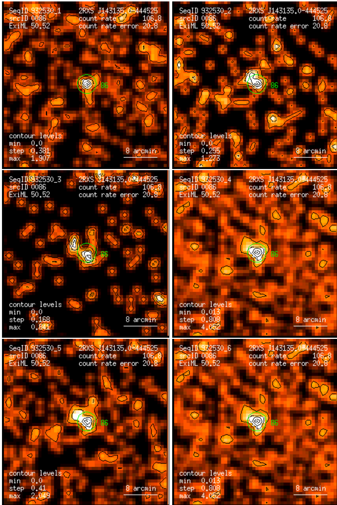
Figure 86: RASS 932530: detection 0086: band rate images, Gaussian filter: (1) PSPC channels 11 – 41, (2) 52 – 90, (3) 91 – 201, (4) 11 – 235, (5) 52 – 201, (6) 11 – 201. Broad band rates in counts/ks. Band rate contour levels in counts/ks/arcmin 2 .
