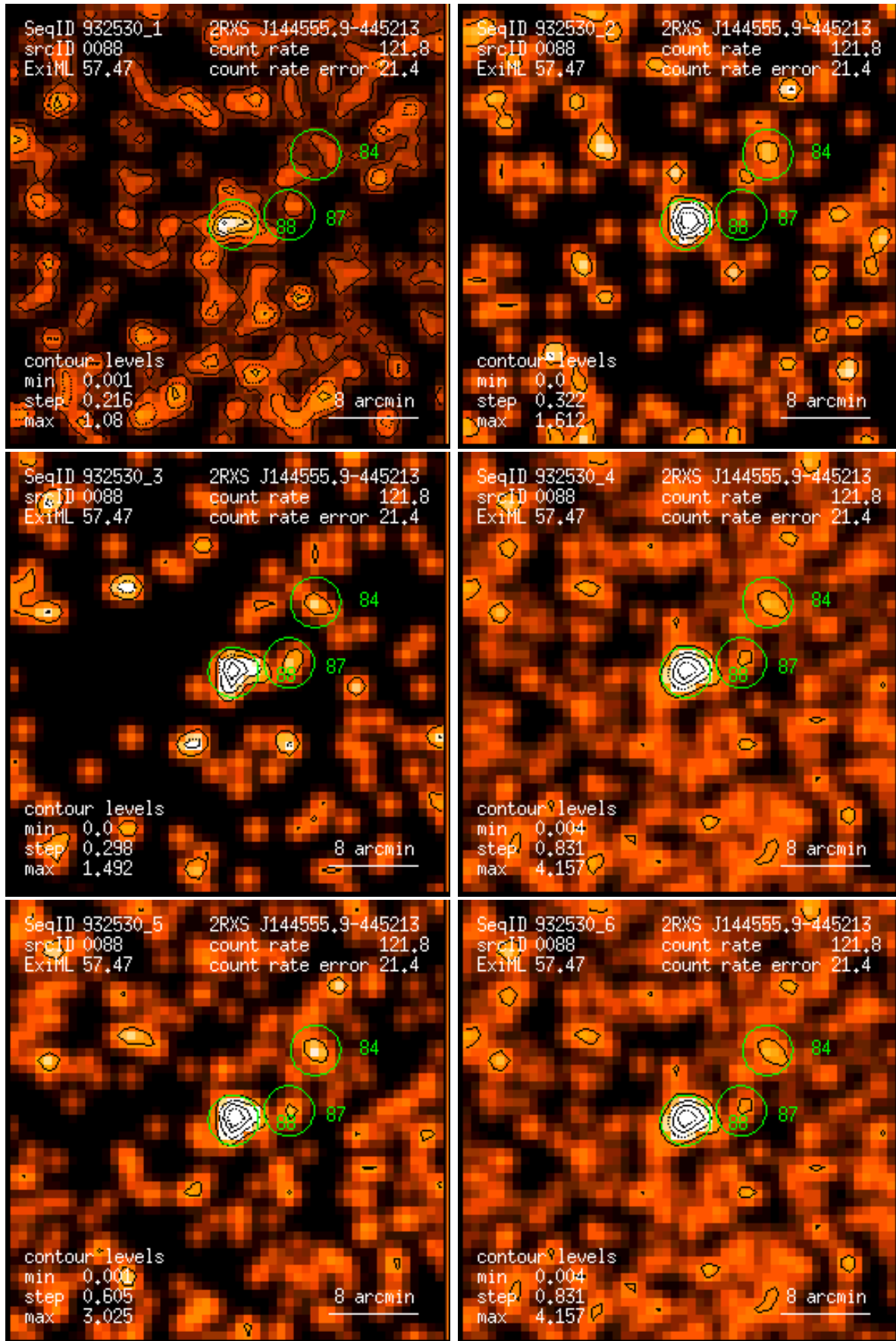
Figure 88: RASS 932530: detection 0088: band rate images, Gaussian filter: (1) PSPC channels 11 – 41, (2) 52 – 90, (3) 91 – 201, (4) 11 – 235, (5) 52 – 201, (6) 11 – 201. Broad band rates in counts/ks. Band rate contour levels in counts/ks/arcmin 2 .
