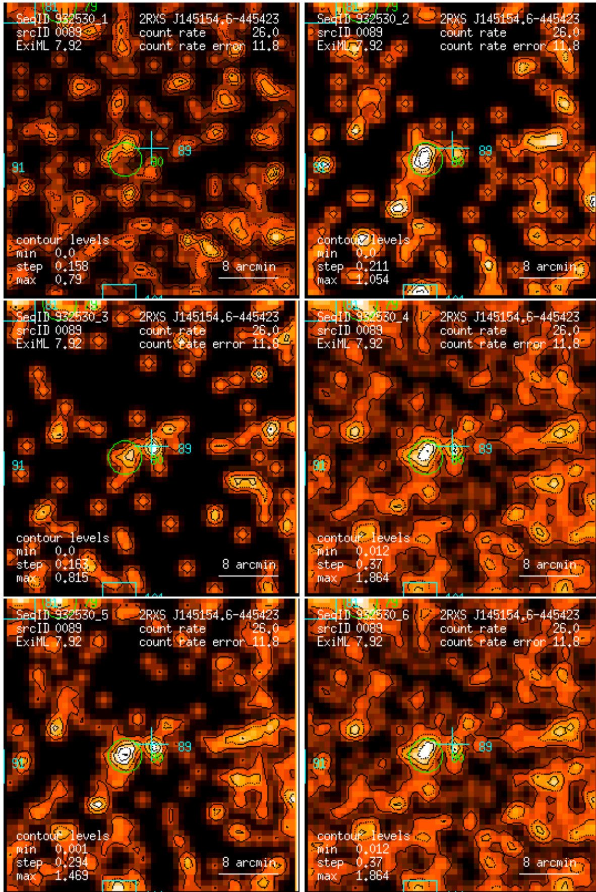
Figure 89: RASS 932530: detection 0089: band rate images, Gaussian filter: (1) PSPC channels 11 – 41, (2) 52 – 90, (3) 91 – 201, (4) 11 – 235, (5) 52 – 201, (6) 11 – 201. Broad band rates in counts/ks. Band rate contour levels in counts/ks/arcmin 2 .
