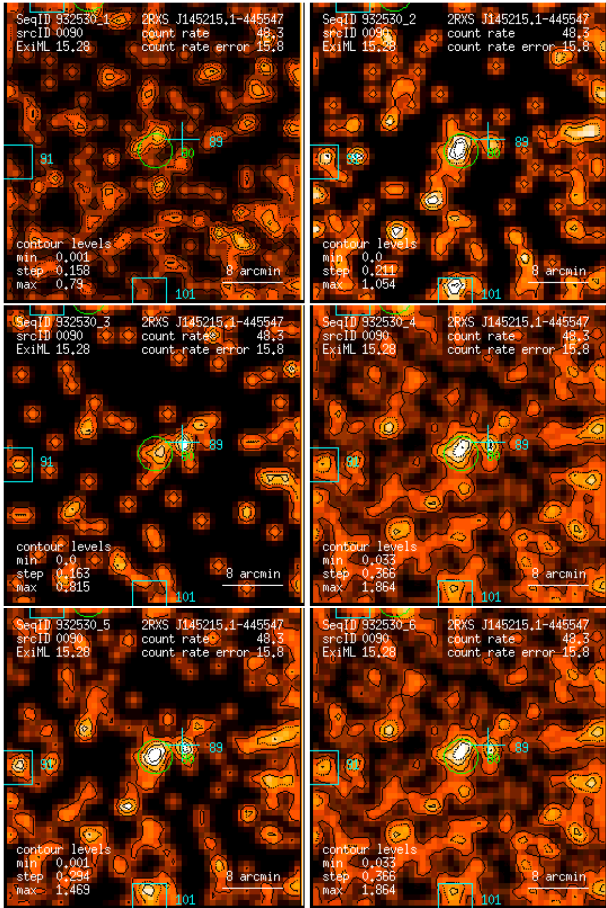
Figure 90: RASS 932530: detection 0090: band rate images, Gaussian filter: (1) PSPC channels 11 – 41, (2) 52 – 90, (3) 91 – 201, (4) 11 – 235, (5) 52 – 201, (6) 11 – 201. Broad band rates in counts/ks. Band rate contour levels in counts/ks/arcmin 2 .
