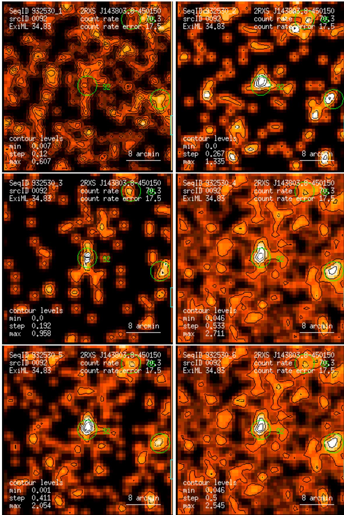
Figure 92: RASS 932530: detection 0092: band rate images, Gaussian filter: (1) PSPC channels 11 – 41, (2) 52 – 90, (3) 91 – 201, (4) 11 – 235, (5) 52 – 201, (6) 11 – 201. Broad band rates in counts/ks. Band rate contour levels in counts/ks/arcmin 2 .
