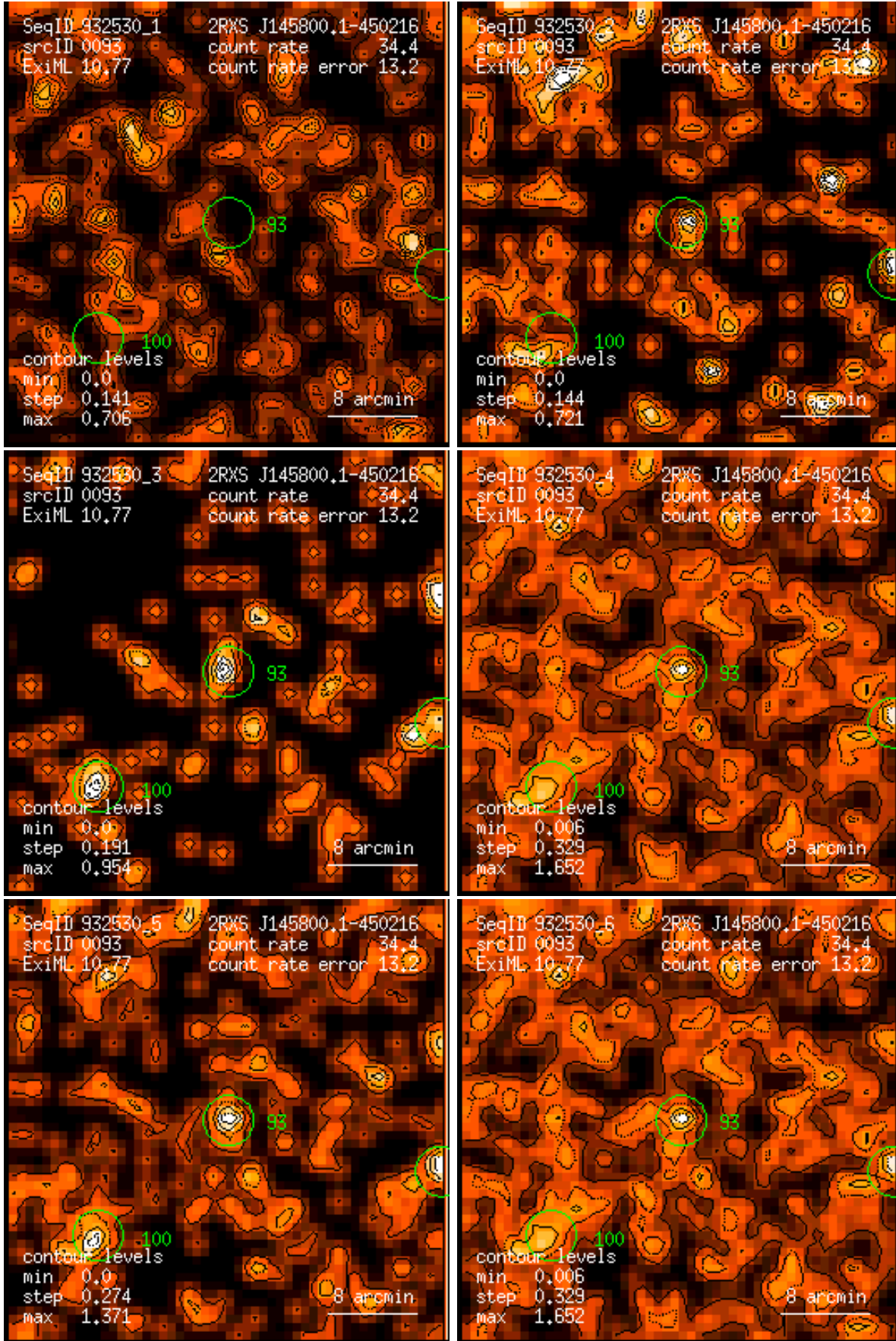
Figure 93: RASS 932530: detection 0093: band rate images, Gaussian filter: (1) PSPC channels 11 – 41, (2) 52 – 90, (3) 91 – 201, (4) 11 – 235, (5) 52 – 201, (6) 11 – 201. Broad band rates in counts/ks. Band rate contour levels in counts/ks/arcmin 2 .
