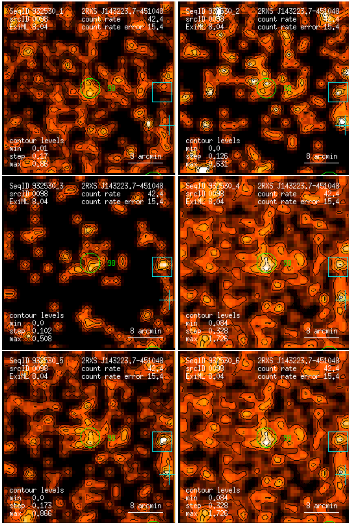
Figure 98: RASS 932530: detection 0098: band rate images, Gaussian filter: (1) PSPC channels 11 – 41, (2) 52 – 90, (3) 91 – 201, (4) 11 – 235, (5) 52 – 201, (6) 11 – 201. Broad band rates in counts/ks. Band rate contour levels in counts/ks/arcmin 2 .
