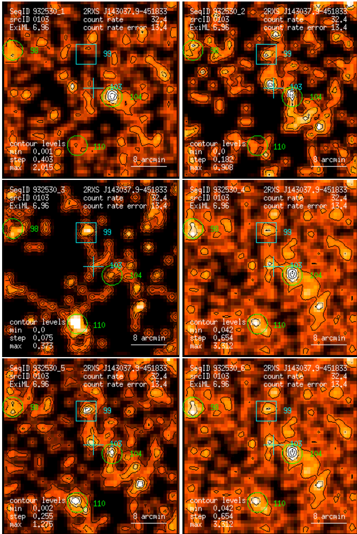
Figure 103: RASS 932530: detection 0103: band rate images, Gaussian filter: (1) PSPC channels 11 – 41, (2) 52 – 90, (3) 91 – 201, (4) 11 – 235, (5) 52 – 201, (6) 11 – 201. Broad band rates in counts/ks. Band rate contour levels in counts/ks/arcmin 2 .
