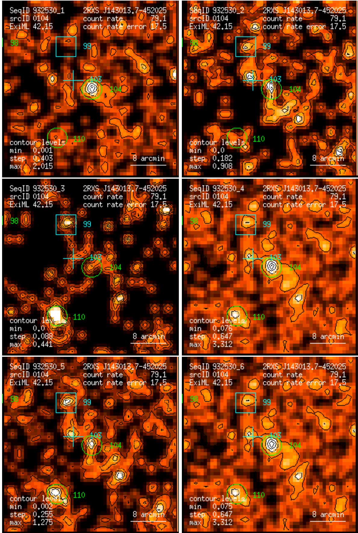
Figure 104: RASS 932530: detection 0104: band rate images, Gaussian filter: (1) PSPC channels 11 – 41, (2) 52 – 90, (3) 91 – 201, (4) 11 – 235, (5) 52 – 201, (6) 11 – 201. Broad band rates in counts/ks. Band rate contour levels in counts/ks/arcmin 2 .
