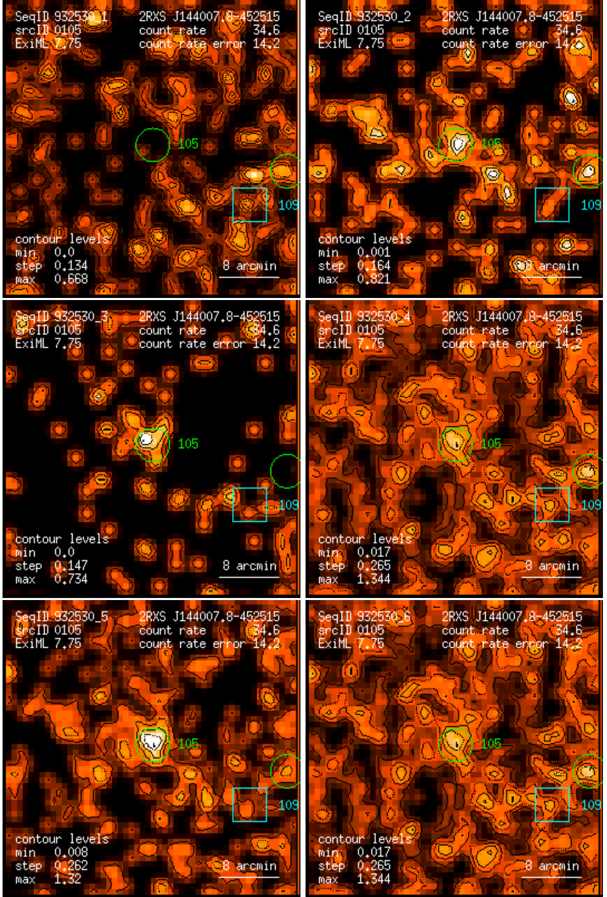
Figure 105: RASS 932530: detection 0105: band rate images, Gaussian filter: (1) PSPC channels 11 – 41, (2) 52 – 90, (3) 91 – 201, (4) 11 – 235, (5) 52 – 201, (6) 11 – 201. Broad band rates in counts/ks. Band rate contour levels in counts/ks/arcmin 2 .
