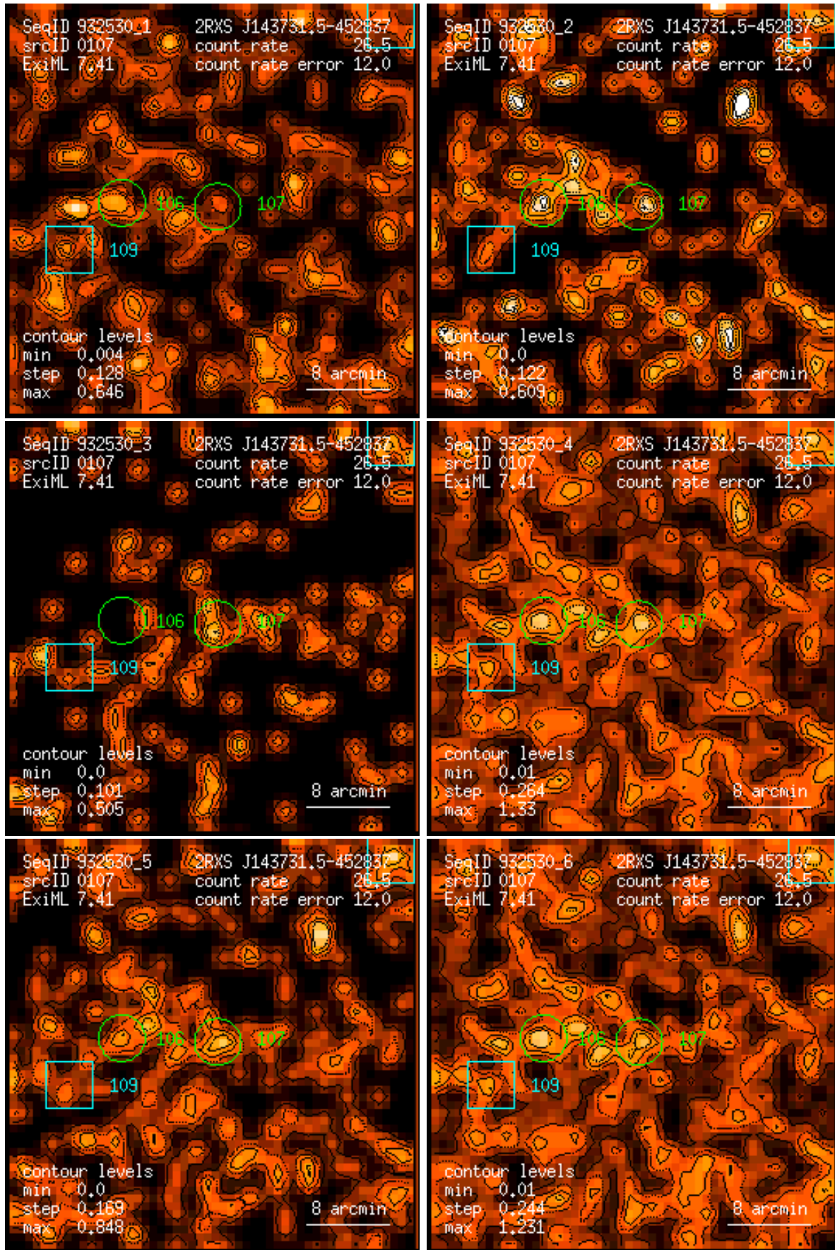
Figure 107: RASS 932530: detection 0107: band rate images, Gaussian filter: (1) PSPC channels 11 – 41, (2) 52 – 90, (3) 91 – 201, (4) 11 – 235, (5) 52 – 201, (6) 11 – 201. Broad band rates in counts/ks. Band rate contour levels in counts/ks/arcmin 2 .
