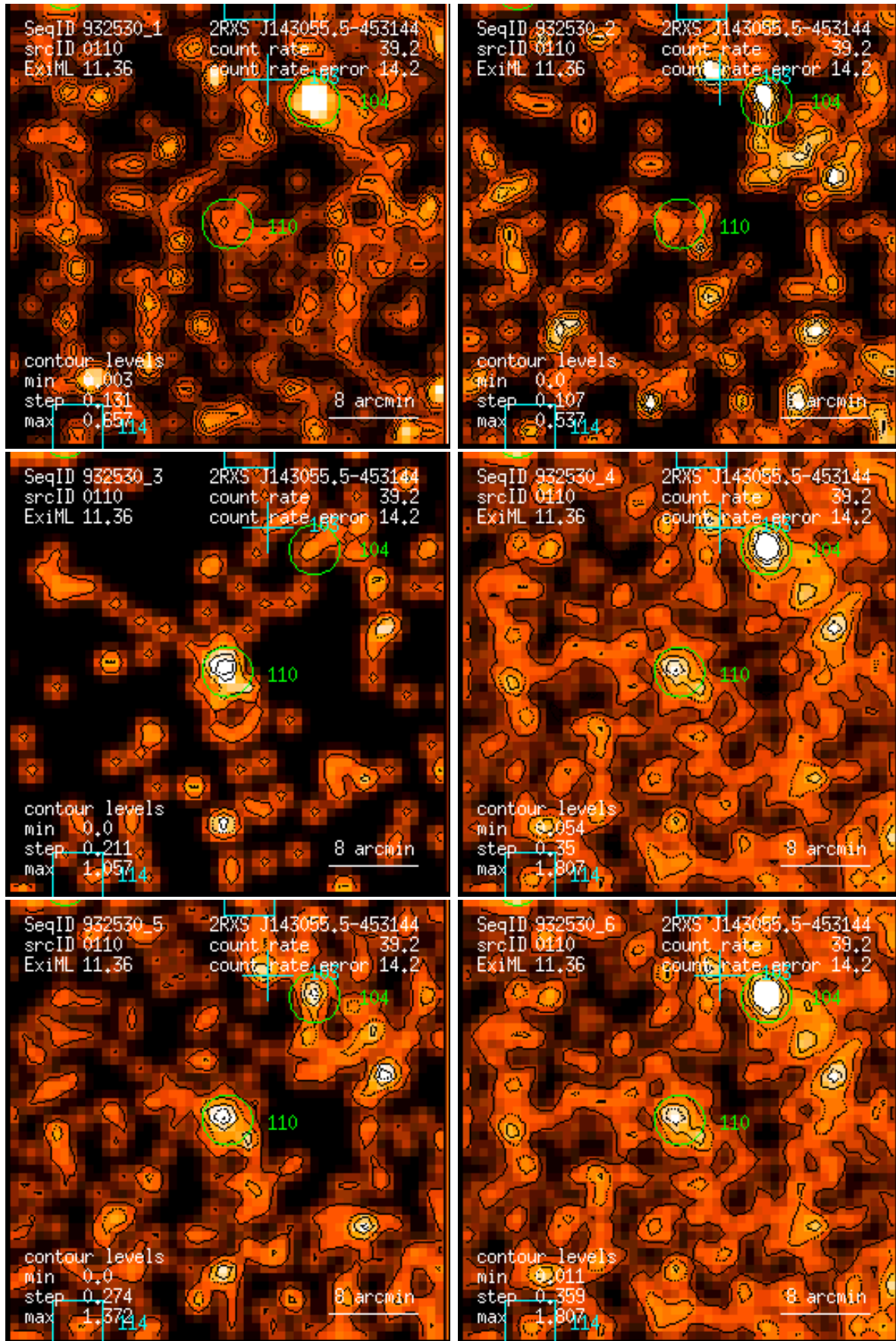
Figure 110: RASS 932530: detection 0110: band rate images, Gaussian filter: (1) PSPC channels 11 – 41, (2) 52 – 90, (3) 91 – 201, (4) 11 – 235, (5) 52 – 201, (6) 11 – 201. Broad band rates in counts/ks. Band rate contour levels in counts/ks/arcmin 2 .
