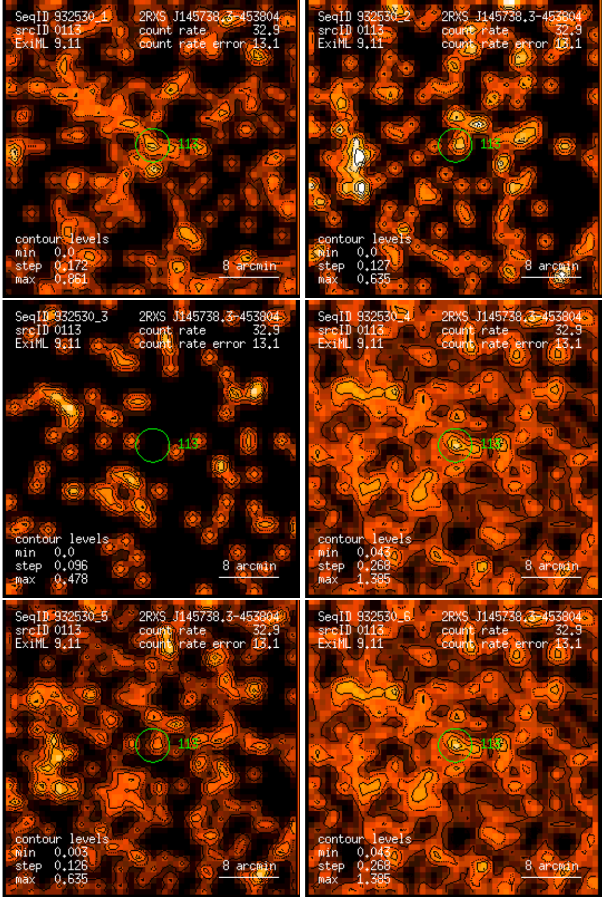
Figure 113: RASS 932530: detection 0113: band rate images, Gaussian filter: (1) PSPC channels 11 – 41, (2) 52 – 90, (3) 91 – 201, (4) 11 – 235, (5) 52 – 201, (6) 11 – 201. Broad band rates in counts/ks. Band rate contour levels in counts/ks/arcmin 2 .
