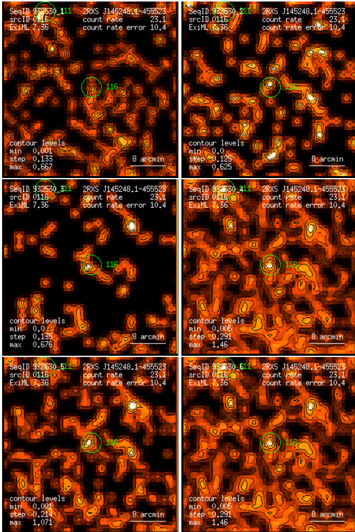
Figure 116: RASS 932530: detection 0116: band rate images, Gaussian filter: (1) PSPC channels 11 – 41, (2) 52 – 90, (3) 91 – 201, (4) 11 – 235, (5) 52 – 201, (6) 11 – 201. Broad band rates in counts/ks. Band rate contour levels in counts/ks/arcmin 2 .
