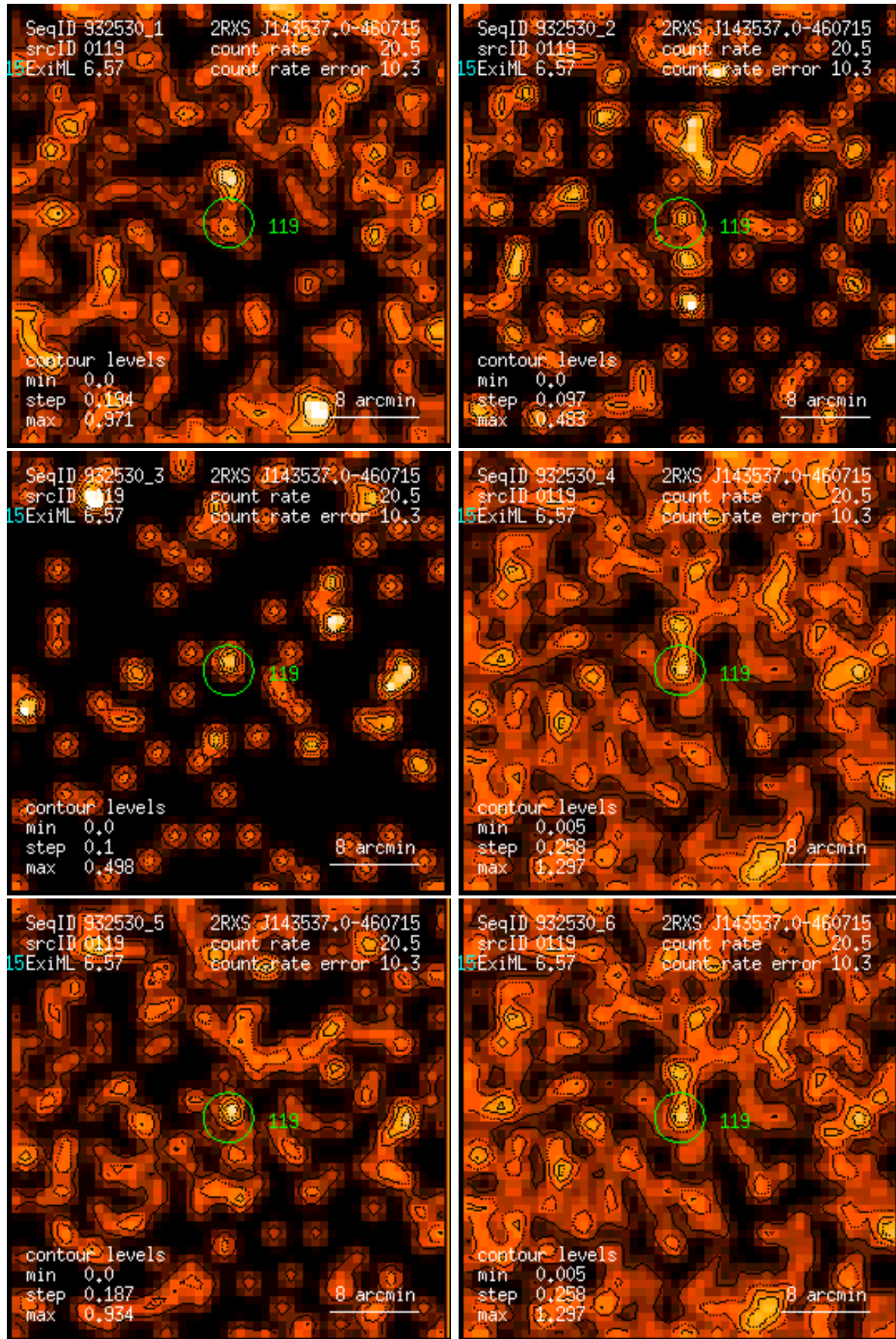
Figure 119: RASS 932530: detection 0119: band rate images, Gaussian filter: (1) PSPC channels 11 – 41, (2) 52 – 90, (3) 91 – 201, (4) 11 – 235, (5) 52 – 201, (6) 11 – 201. Broad band rates in counts/ks. Band rate contour levels in counts/ks/arcmin 2 .
