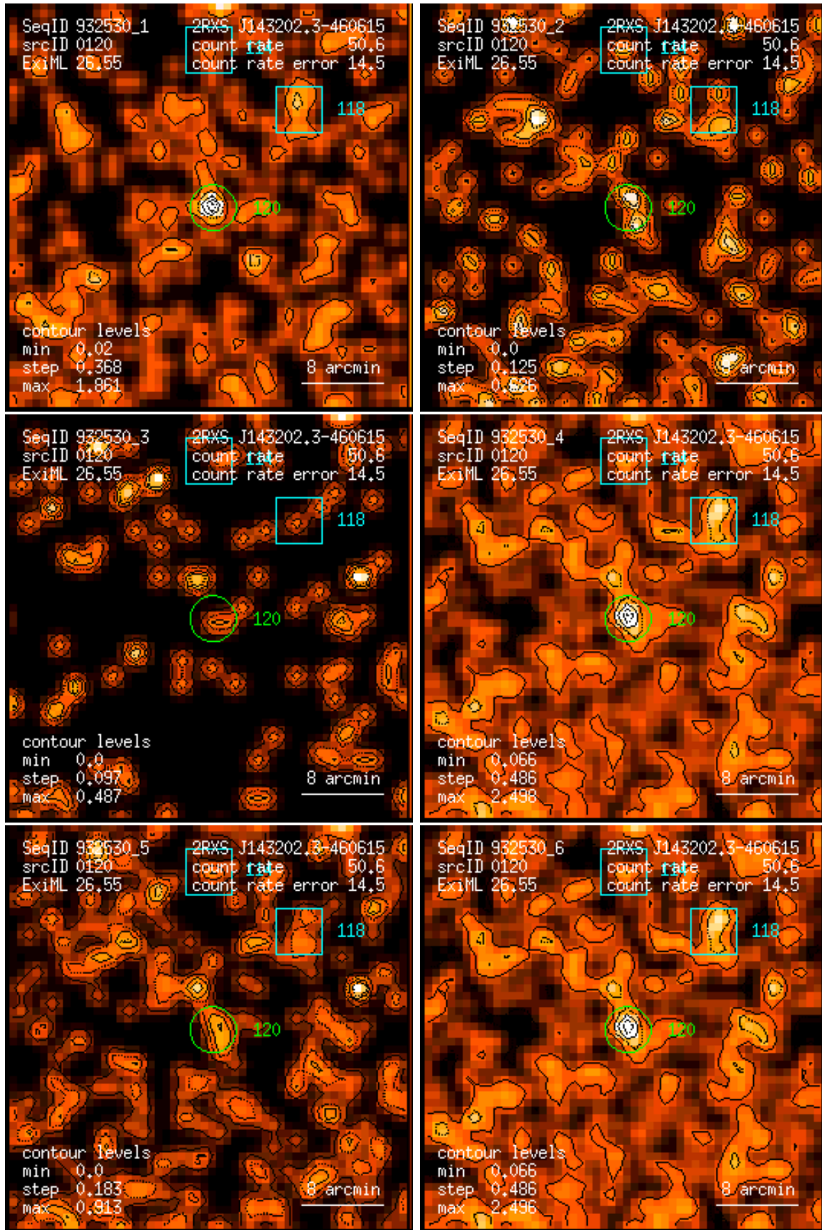
Figure 120: RASS 932530: detection 0120: band rate images, Gaussian filter: (1) PSPC channels 11 – 41, (2) 52 – 90, (3) 91 – 201, (4) 11 – 235, (5) 52 – 201, (6) 11 – 201. Broad band rates in counts/ks. Band rate contour levels in counts/ks/arcmin 2 .
