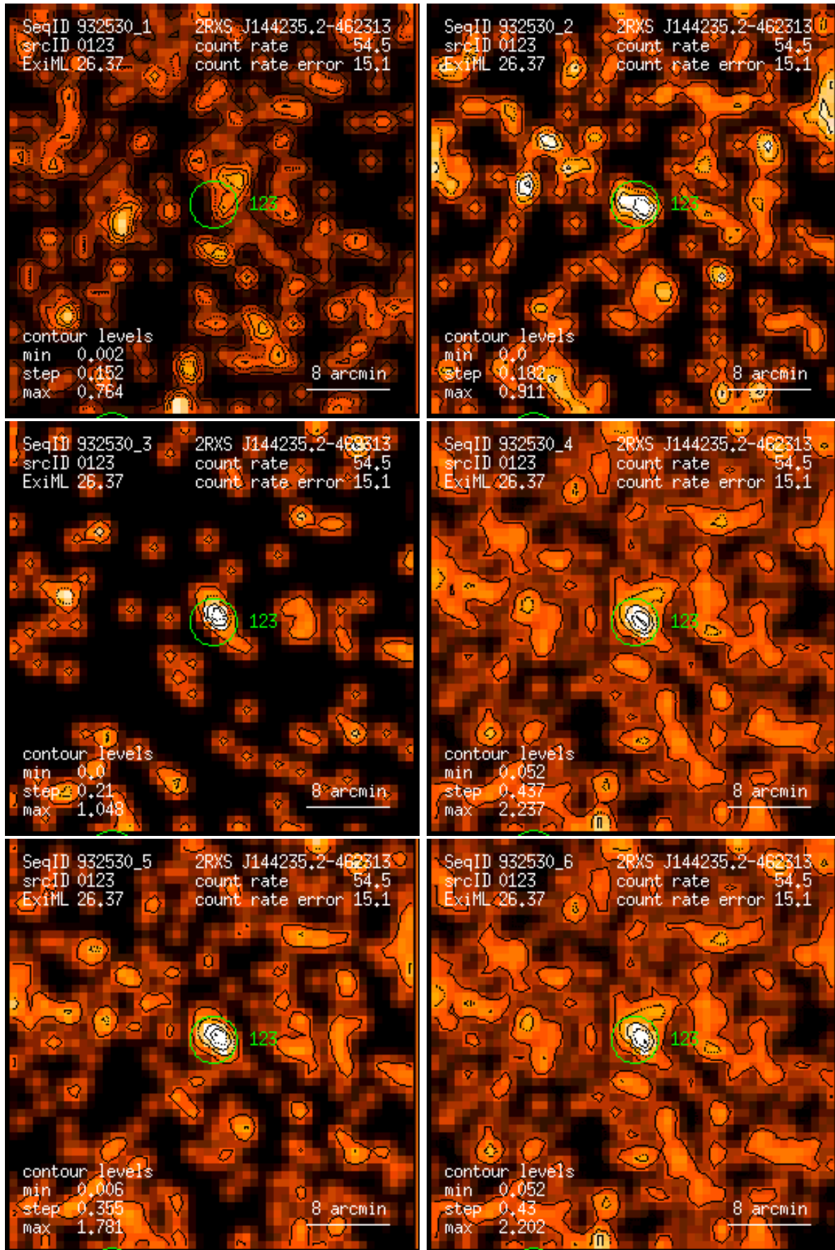
Figure 123: RASS 932530: detection 0123: band rate images, Gaussian filter: (1) PSPC channels 11 – 41, (2) 52 – 90, (3) 91 – 201, (4) 11 – 235, (5) 52 – 201, (6) 11 – 201. Broad band rates in counts/ks. Band rate contour levels in counts/ks/arcmin 2 .
