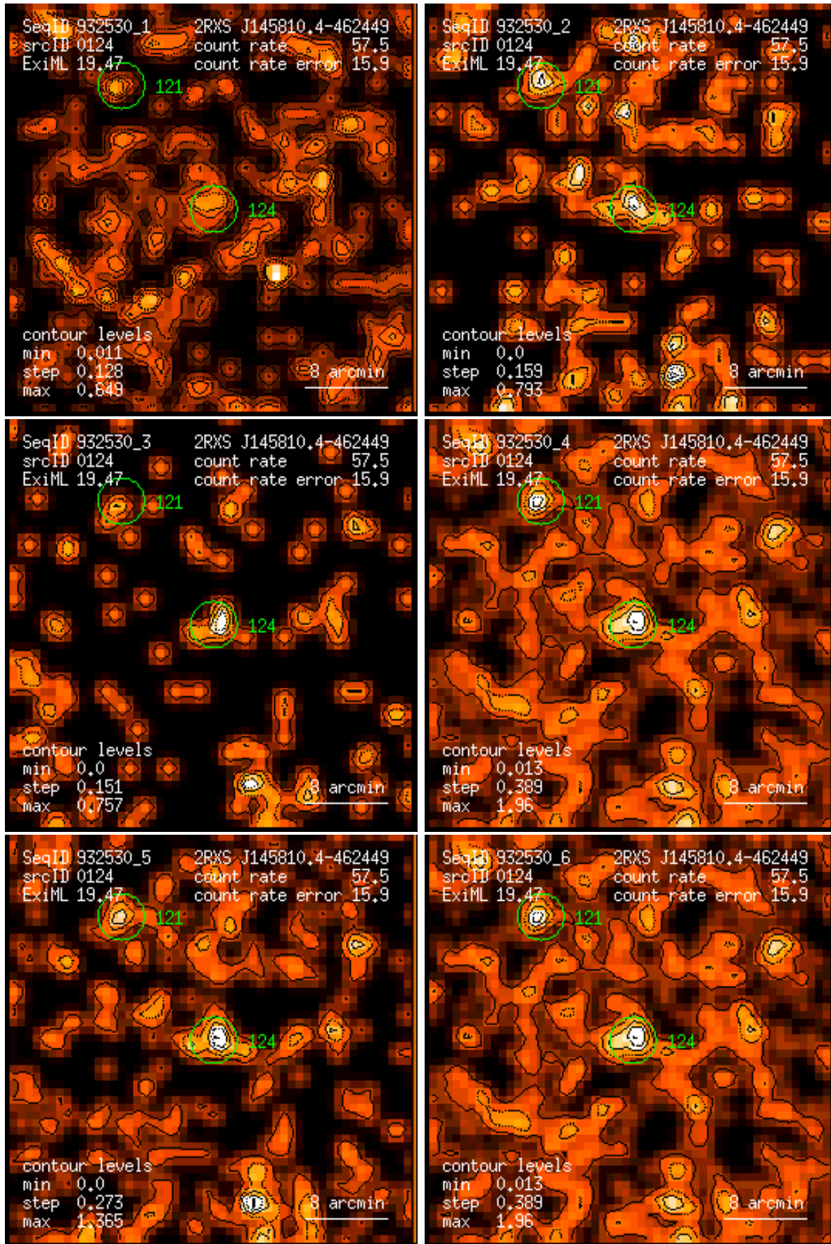
Figure 124: RASS 932530: detection 0124: band rate images, Gaussian filter: (1) PSPC channels 11 – 41, (2) 52 – 90, (3) 91 – 201, (4) 11 – 235, (5) 52 – 201, (6) 11 – 201. Broad band rates in counts/ks. Band rate contour levels in counts/ks/arcmin 2 .
