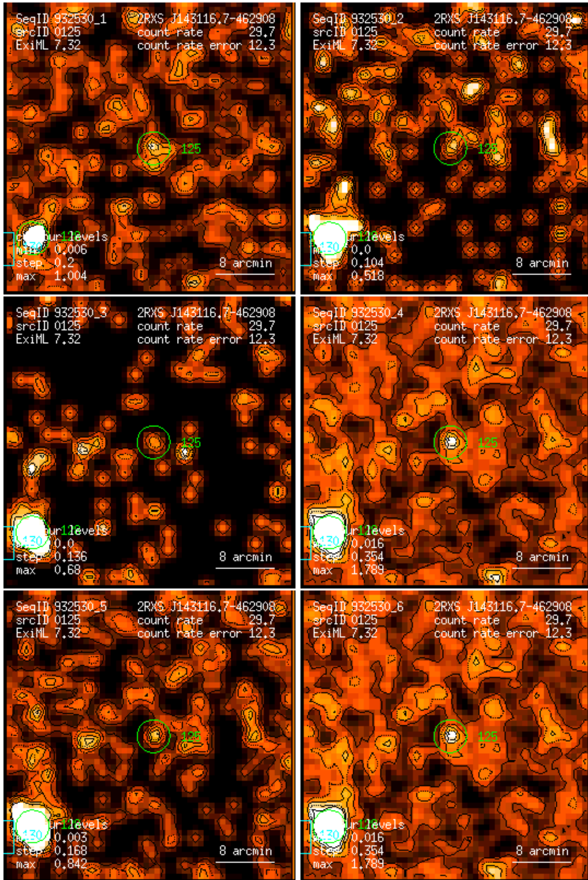
Figure 125: RASS 932530: detection 0125: band rate images, Gaussian filter: (1) PSPC channels 11 – 41, (2) 52 – 90, (3) 91 – 201, (4) 11 – 235, (5) 52 – 201, (6) 11 – 201. Broad band rates in counts/ks. Band rate contour levels in counts/ks/arcmin 2 .
