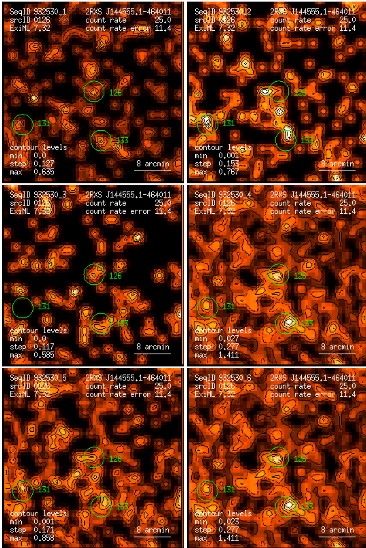
Figure 126: RASS 932530: detection 0126: band rate images, Gaussian filter: (1) PSPC channels 11 – 41, (2) 52 – 90, (3) 91 – 201, (4) 11 – 235, (5) 52 – 201, (6) 11 – 201. Broad band rates in counts/ks. Band rate contour levels in counts/ks/arcmin 2 .
