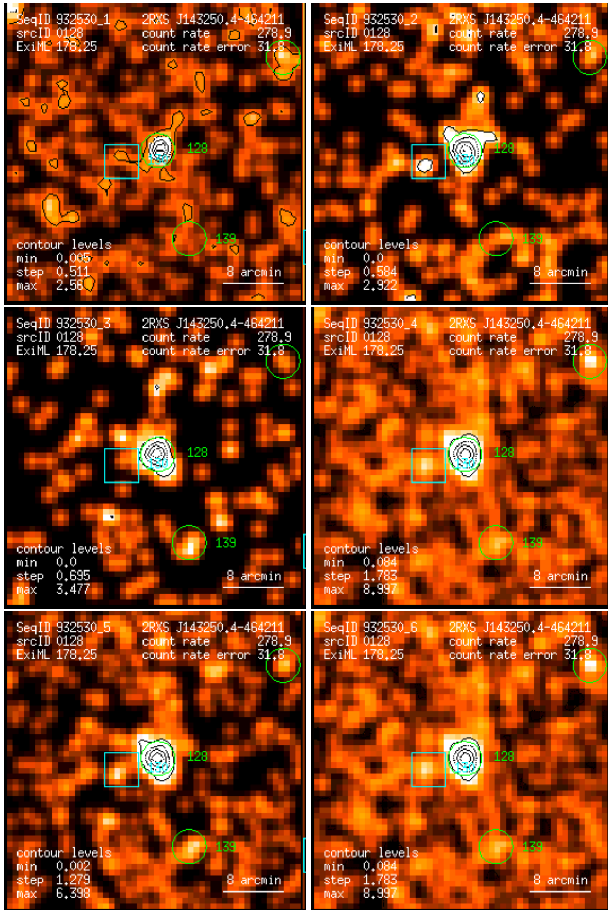
Figure 128: RASS 932530: detection 0128: band rate images, Gaussian filter: (1) PSPC channels 11 – 41, (2) 52 – 90, (3) 91 – 201, (4) 11 – 235, (5) 52 – 201, (6) 11 – 201. Broad band rates in counts/ks. Band rate contour levels in counts/ks/arcmin 2 .
