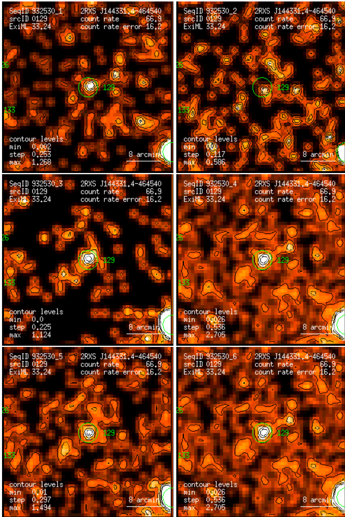
Figure 129: RASS 932530: detection 0129: band rate images, Gaussian filter: (1) PSPC channels 11 – 41, (2) 52 – 90, (3) 91 – 201, (4) 11 – 235, (5) 52 – 201, (6) 11 – 201. Broad band rates in counts/ks. Band rate contour levels in counts/ks/arcmin 2 .
