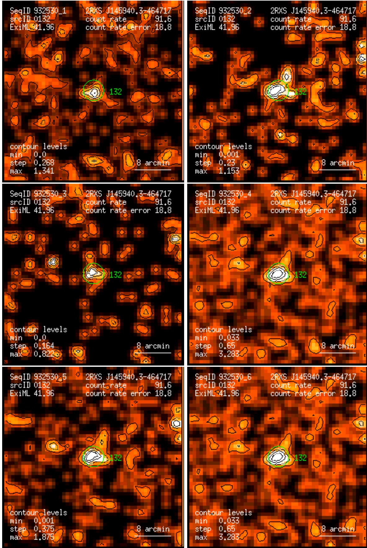
Figure 132: RASS 932530: detection 0132: band rate images, Gaussian filter: (1) PSPC channels 11 – 41, (2) 52 – 90, (3) 91 – 201, (4) 11 – 235, (5) 52 – 201, (6) 11 – 201. Broad band rates in counts/ks. Band rate contour levels in counts/ks/arcmin 2 .
