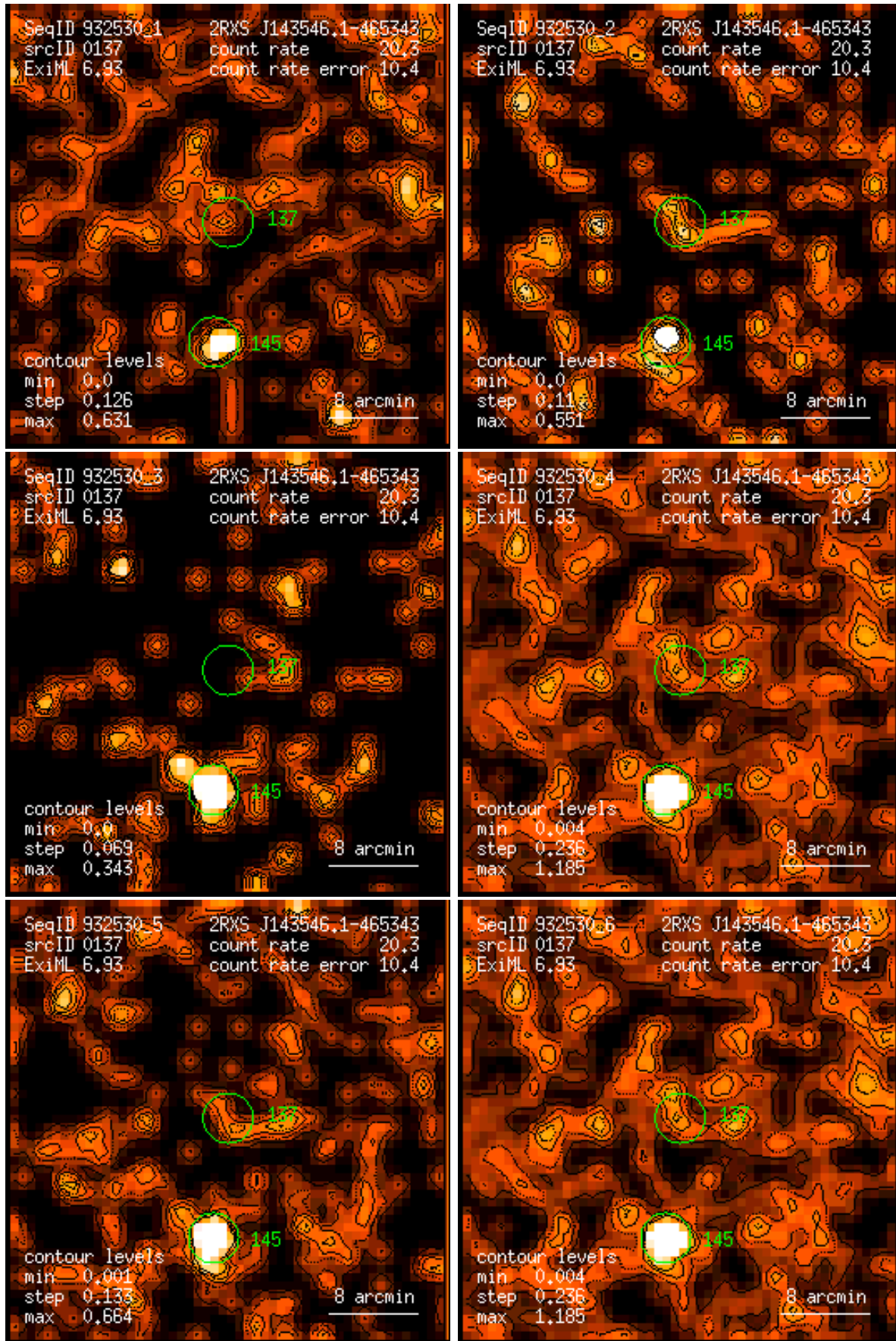
Figure 137: RASS 932530: detection 0137: band rate images, Gaussian filter: (1) PSPC channels 11 – 41, (2) 52 – 90, (3) 91 – 201, (4) 11 – 235, (5) 52 – 201, (6) 11 – 201. Broad band rates in counts/ks. Band rate contour levels in counts/ks/arcmin 2 .
