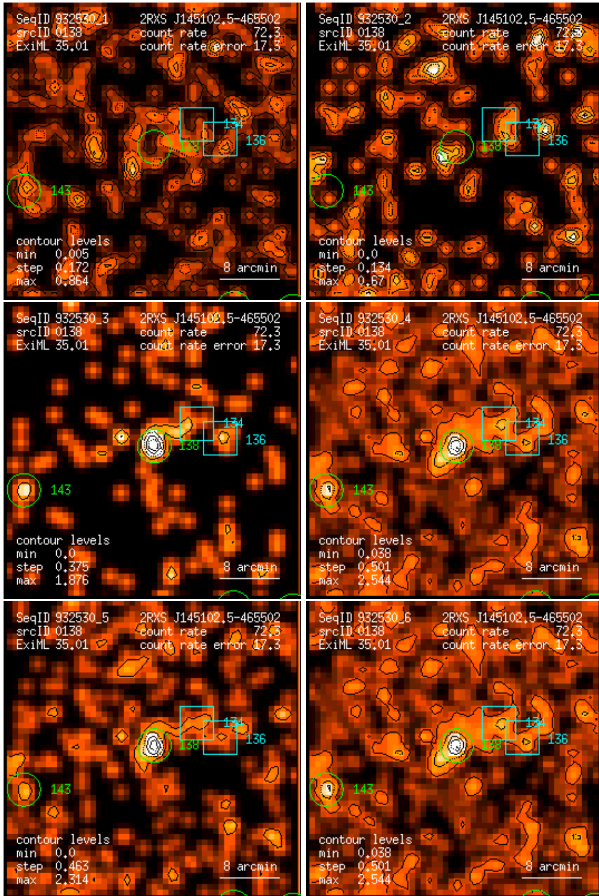
Figure 138: RASS 932530: detection 0138: band rate images, Gaussian filter: (1) PSPC channels 11 – 41, (2) 52 – 90, (3) 91 – 201, (4) 11 – 235, (5) 52 – 201, (6) 11 – 201. Broad band rates in counts/ks. Band rate contour levels in counts/ks/arcmin 2 .
