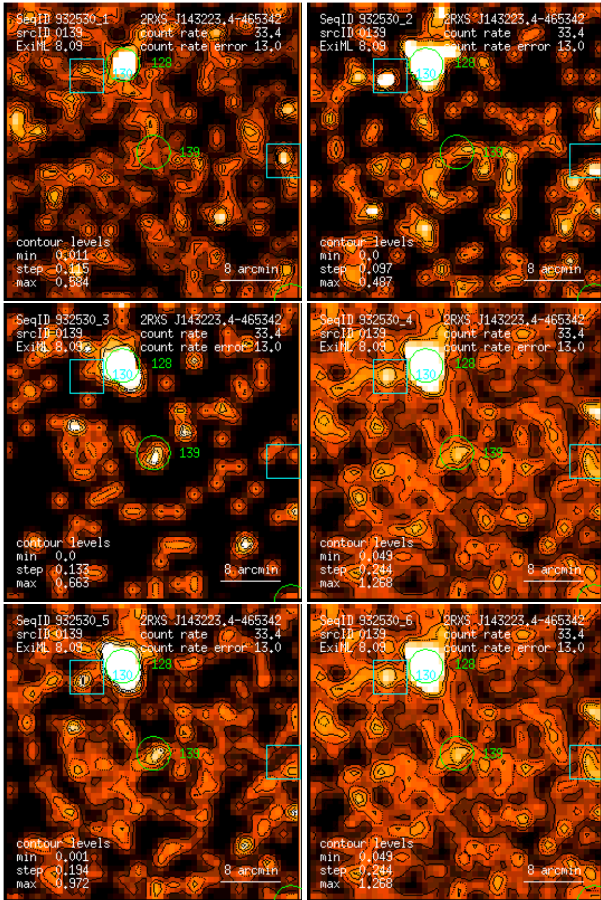
Figure 139: RASS 932530: detection 0139: band rate images, Gaussian filter: (1) PSPC channels 11 – 41, (2) 52 – 90, (3) 91 – 201, (4) 11 – 235, (5) 52 – 201, (6) 11 – 201. Broad band rates in counts/ks. Band rate contour levels in counts/ks/arcmin 2 .
