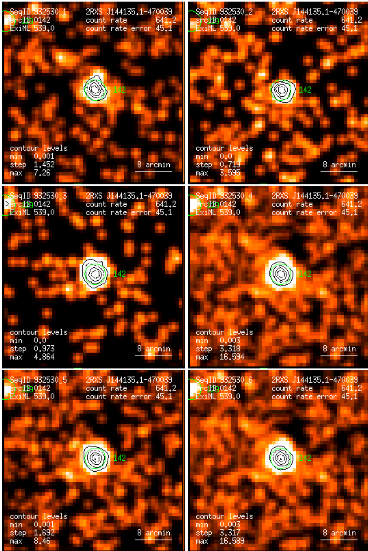
Figure 142: RASS 932530: detection 0142: band rate images, Gaussian filter: (1) PSPC channels 11 – 41, (2) 52 – 90, (3) 91 – 201, (4) 11 – 235, (5) 52 – 201, (6) 11 – 201. Broad band rates in counts/ks. Band rate contour levels in counts/ks/arcmin 2 .
