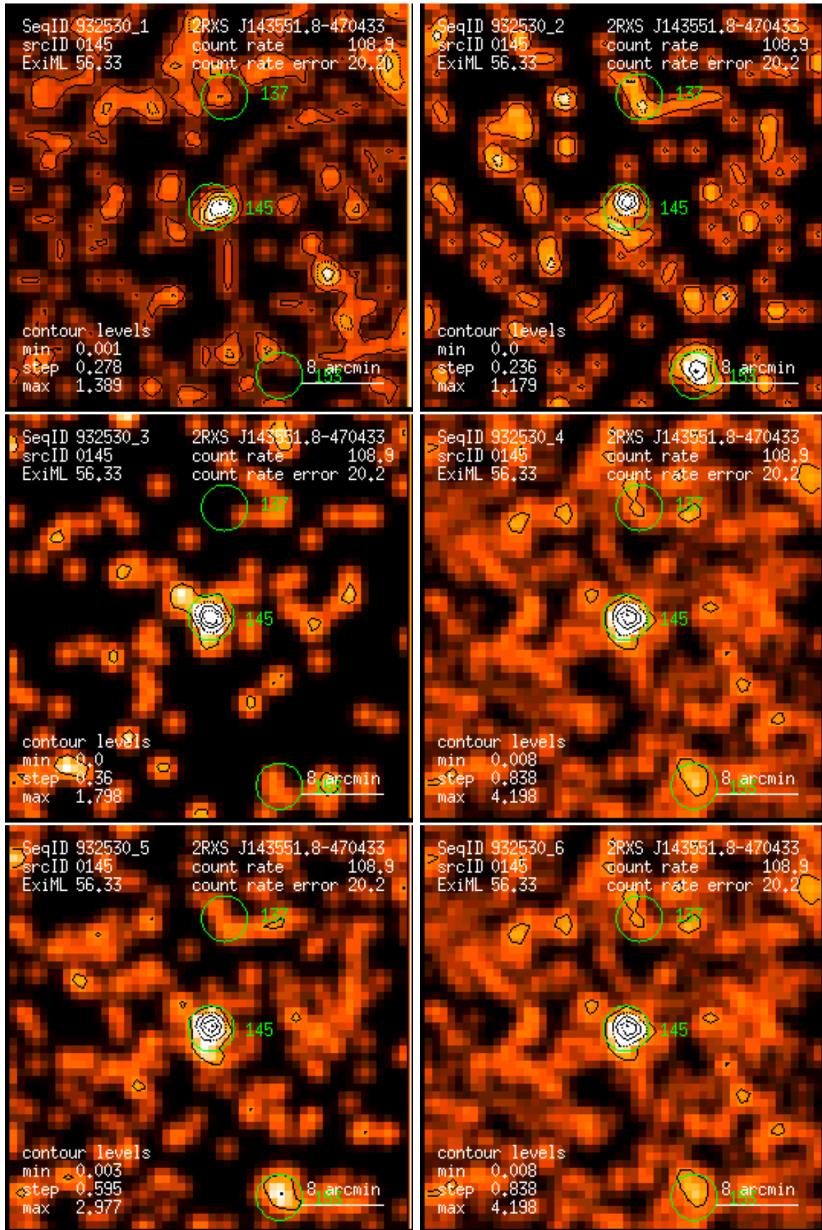
Figure 145: RASS 932530: detection 0145: band rate images, Gaussian filter: (1) PSPC channels 11 – 41, (2) 52 – 90, (3) 91 – 201, (4) 11 – 235, (5) 52 – 201, (6) 11 – 201. Broad band rates in counts/ks. Band rate contour levels in counts/ks/arcmin 2 .
