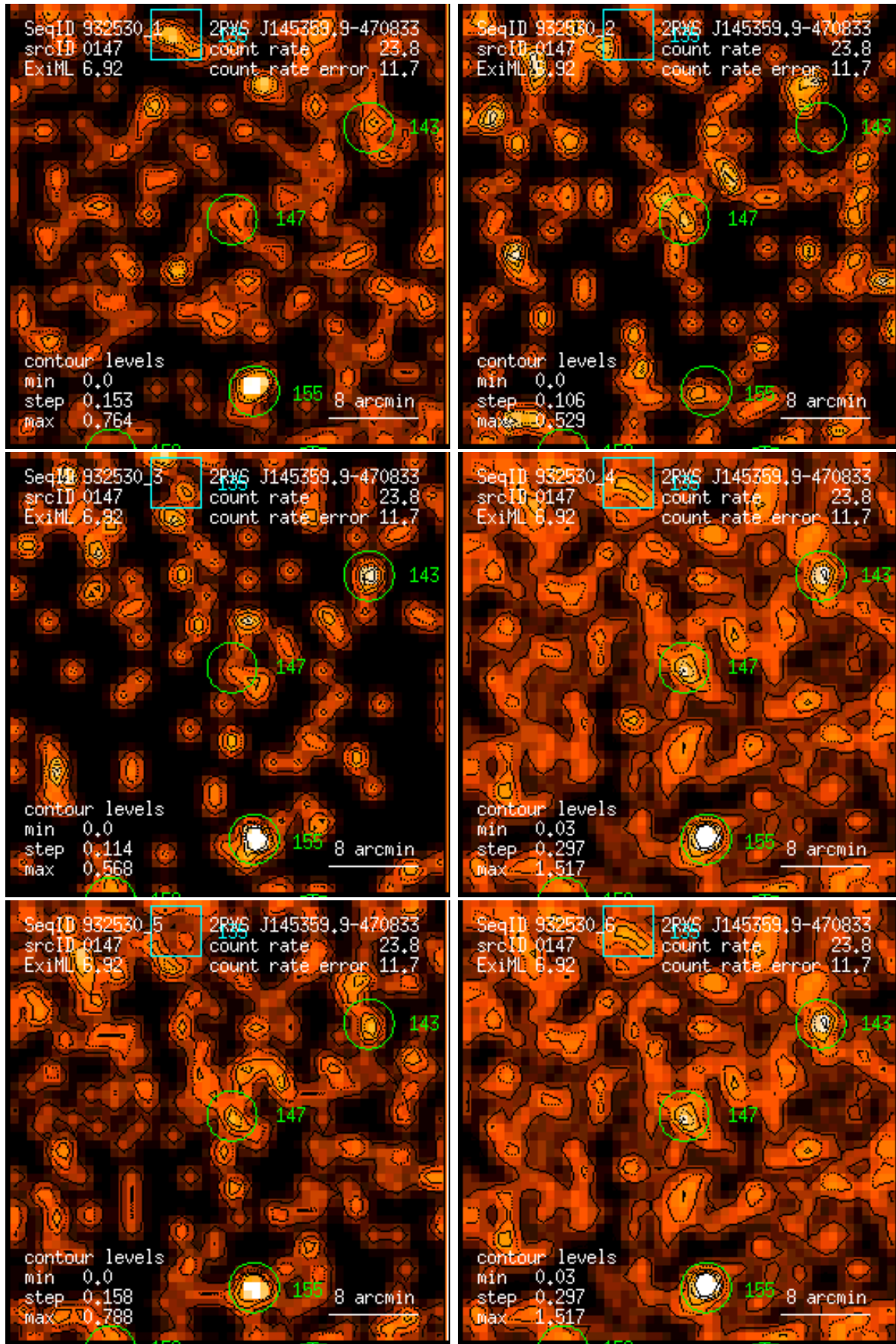
Figure 147: RASS 932530: detection 0147: band rate images, Gaussian filter: (1) PSPC channels 11 – 41, (2) 52 – 90, (3) 91 – 201, (4) 11 – 235, (5) 52 – 201, (6) 11 – 201. Broad band rates in counts/ks. Band rate contour levels in counts/ks/arcmin 2 .
