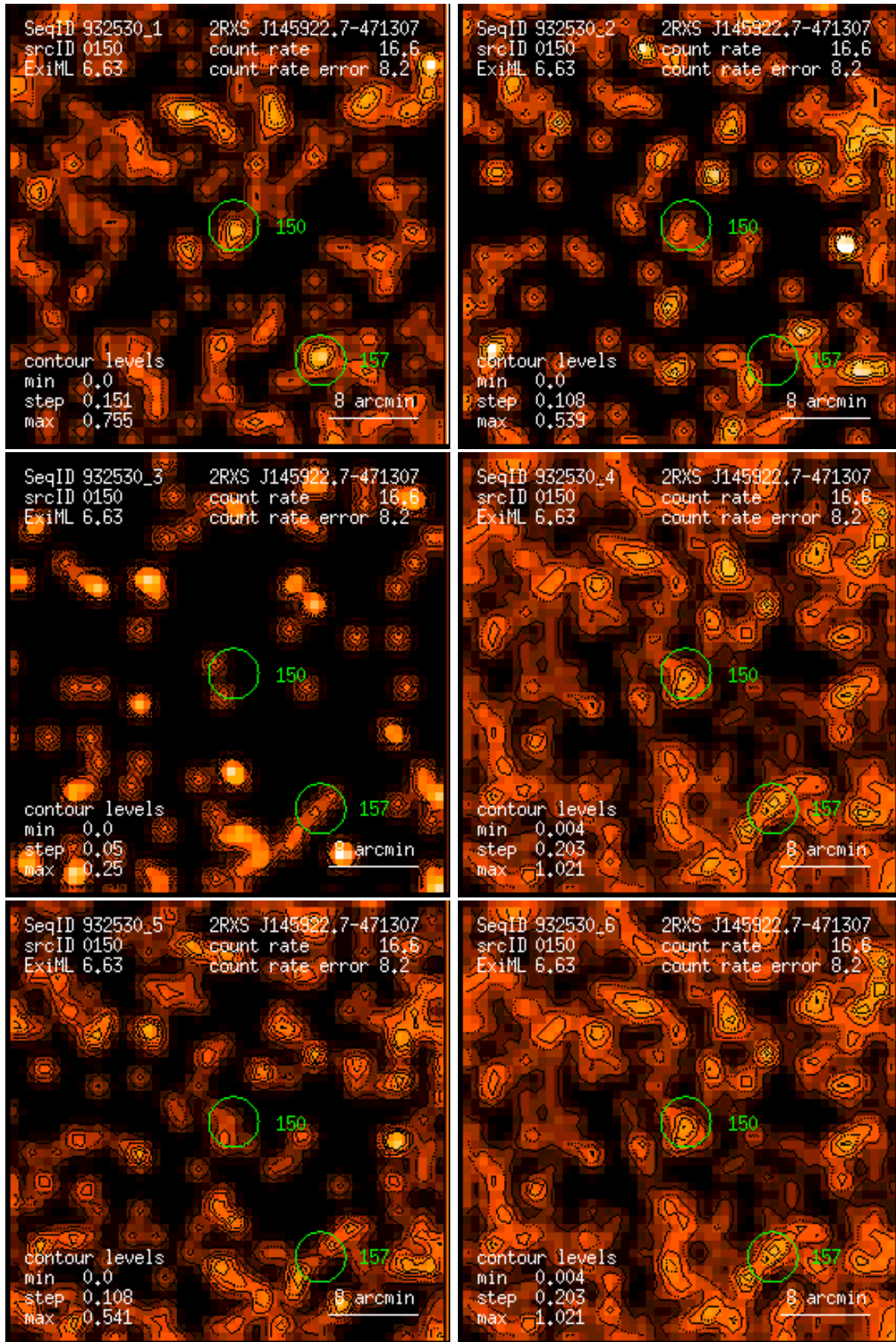
Figure 150: RASS 932530: detection 0150: band rate images, Gaussian filter: (1) PSPC channels 11 – 41, (2) 52 – 90, (3) 91 – 201, (4) 11 – 235, (5) 52 – 201, (6) 11 – 201. Broad band rates in counts/ks. Band rate contour levels in counts/ks/arcmin 2 .
