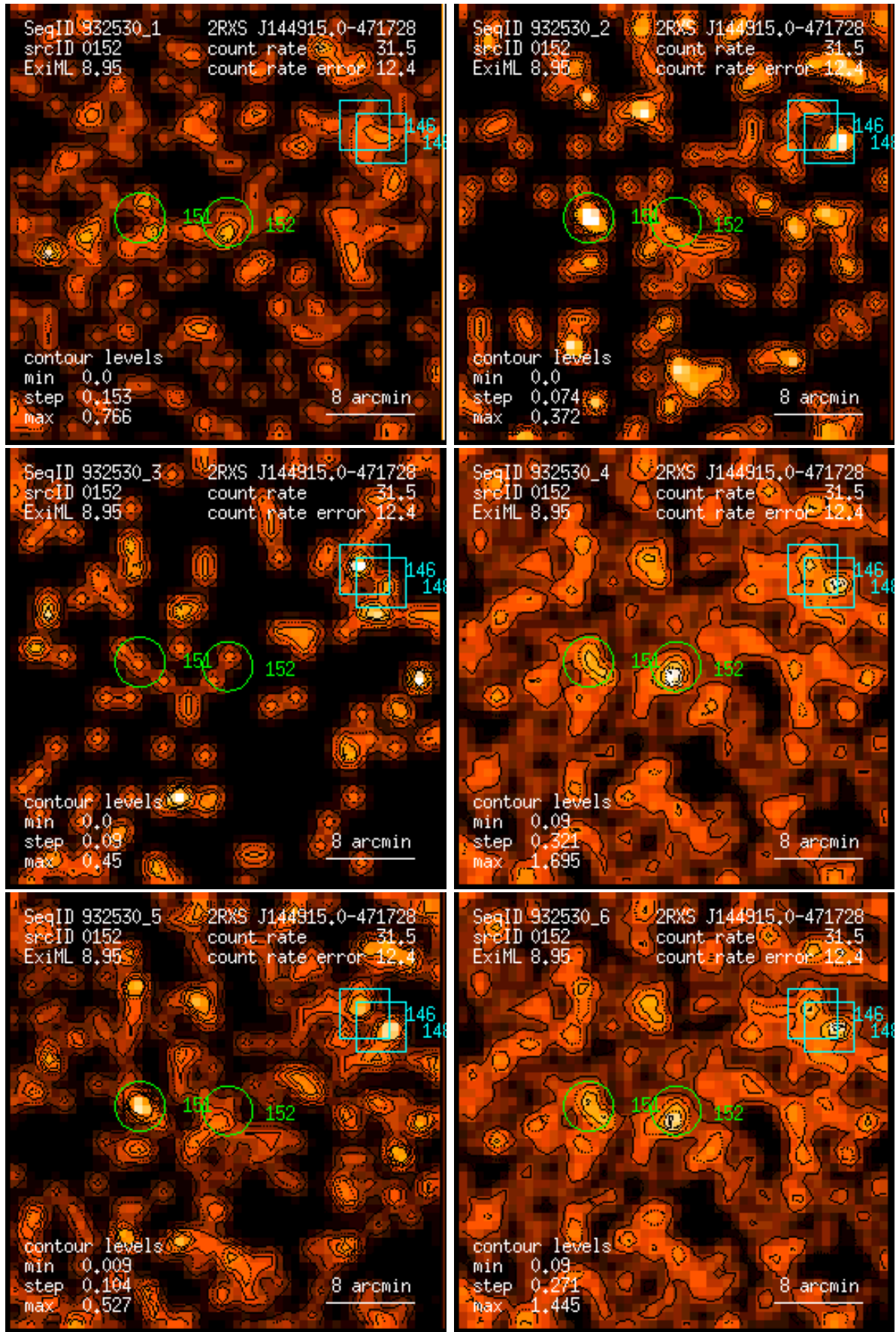
Figure 152: RASS 932530: detection 0152: band rate images, Gaussian filter: (1) PSPC channels 11 – 41, (2) 52 – 90, (3) 91 – 201, (4) 11 – 235, (5) 52 – 201, (6) 11 – 201. Broad band rates in counts/ks. Band rate contour levels in counts/ks/arcmin 2 .
