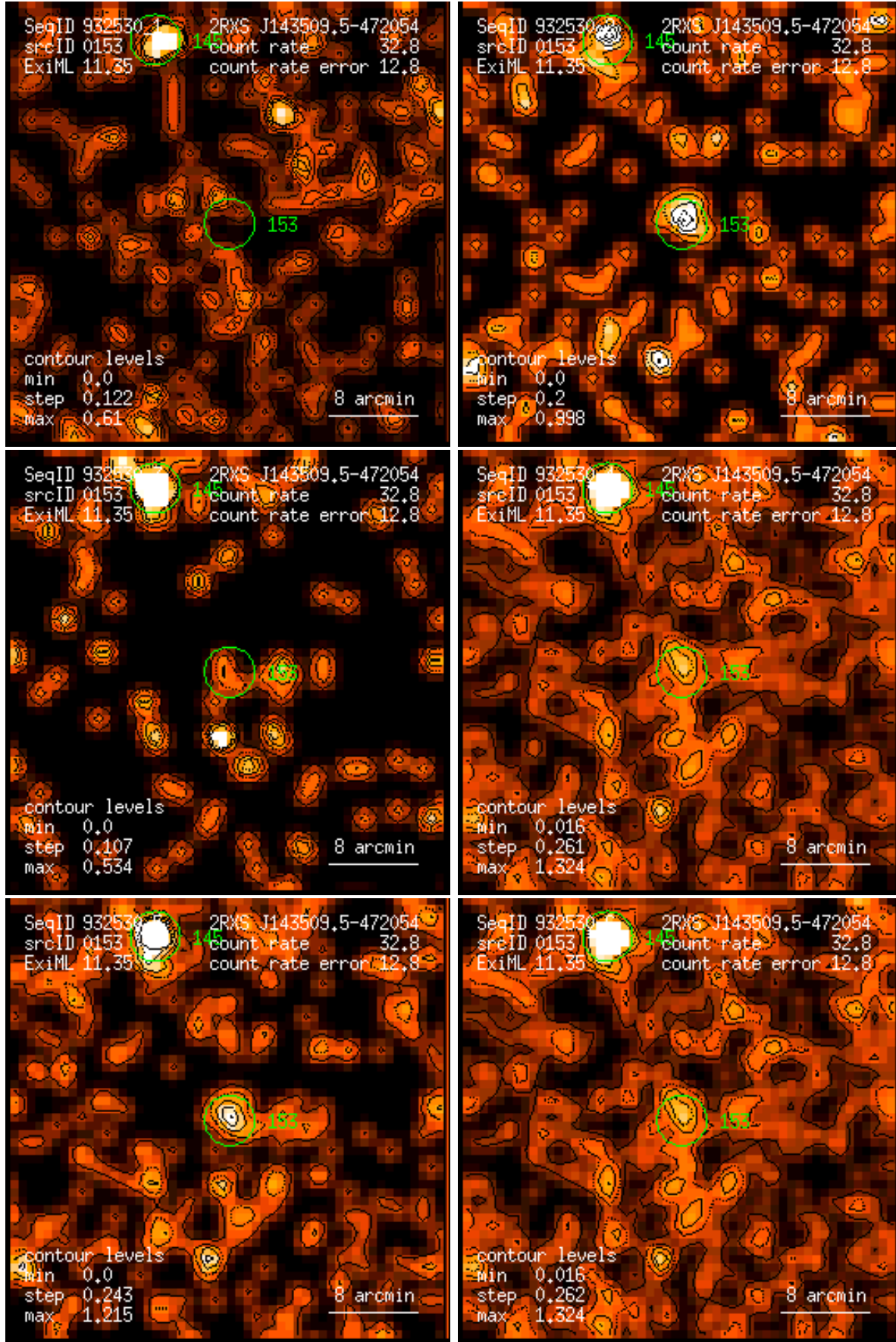
Figure 153: RASS 932530: detection 0153: band rate images, Gaussian filter: (1) PSPC channels 11 – 41, (2) 52 – 90, (3) 91 – 201, (4) 11 – 235, (5) 52 – 201, (6) 11 – 201. Broad band rates in counts/ks. Band rate contour levels in counts/ks/arcmin 2 .
