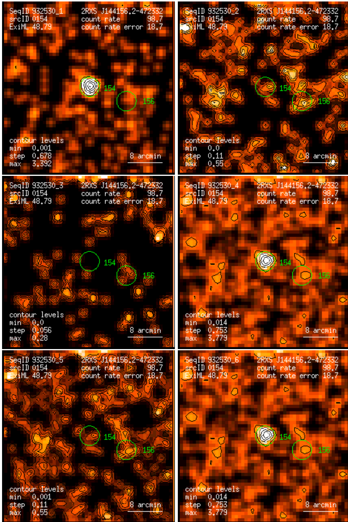
Figure 154: RASS 932530: detection 0154: band rate images, Gaussian filter: (1) PSPC channels 11 – 41, (2) 52 – 90, (3) 91 – 201, (4) 11 – 235, (5) 52 – 201, (6) 11 – 201. Broad band rates in counts/ks. Band rate contour levels in counts/ks/arcmin 2 .
